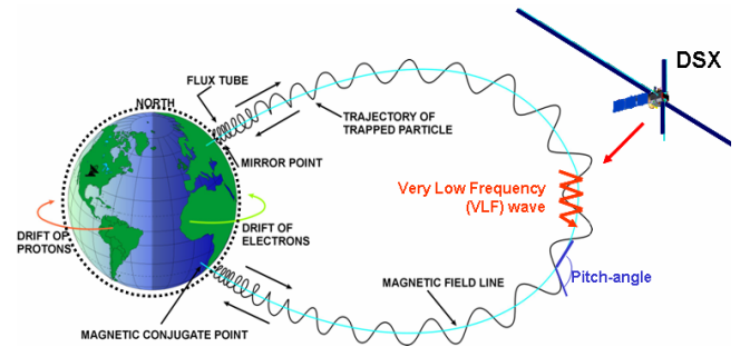
Figure 8. VLF wave particle interaction process.
