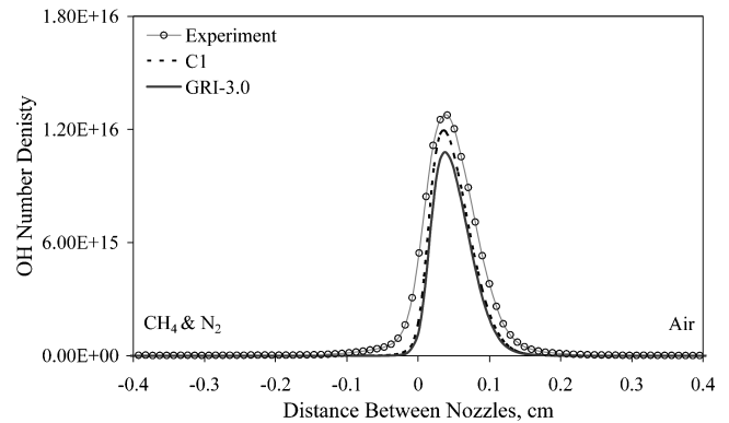
Fig. 17 Comparison of OH number density distributions with 0 W of plasma power addition at a strain rate of 83.3 \text{ s}^{-1} .
