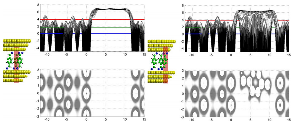
Fig. 1: Potential profiles for xylyldithiol molecule between gold leads as calculated using a plane wave basis. The left figures represent the situation in which no molecule is attached, so only the Au atoms appear on the left and right sides of the potential (top curves). The figure on the left indicates where the plot is taken (shaded region through the molecule, which is absent). The lower panel is a “top down” view of the atomic arrangement. The right figures have the molecule in place, and the modification due to the atoms of the molecule is evident. The green line is the Fermi level, the red line is the expected LUMO level, and the blue line is the HOMO level. The horizontal axes in the four plots is the position, in Angstrom, relative to the center of the last Au layer on the left.
