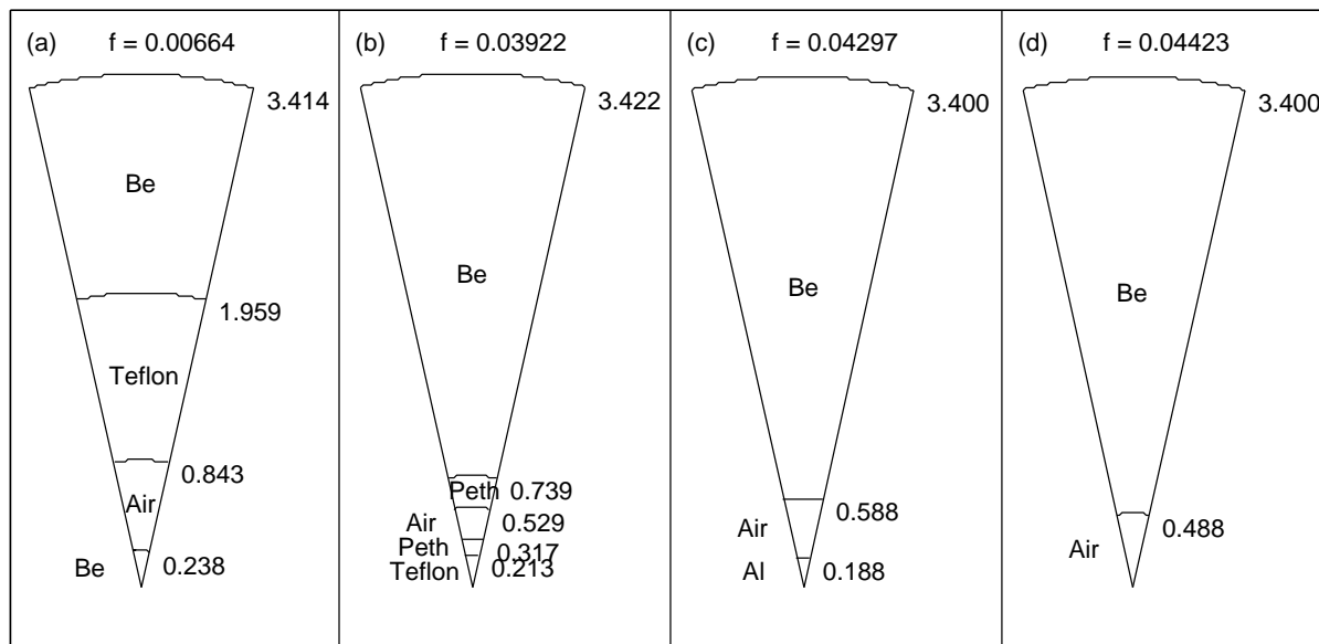
Figure 5: I (inconclusive) rating example for test 3e showing the true object (a), the best three reconstructions (b-d), and corresponding objective function values f . Radial positions of layer boundaries are given in centimeters and material identifications are provided within or near each layer.
