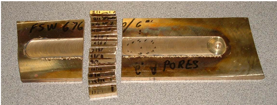
Figure 3.2 Sectioned Sample
