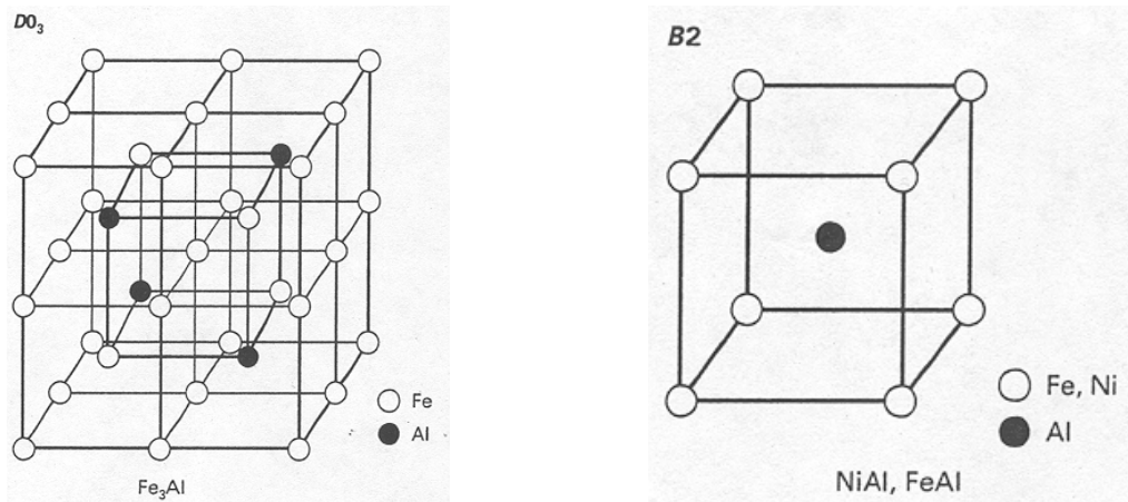
Figure 2.2b: DO_3 and B_2 crystal structures. \kappa_{II} and \kappa_{IV} have a Fe_3Al composition with a DO_3 crystal structure, while \kappa_{III} exhibits a NiAl composition with a B_2 crystal structure.
