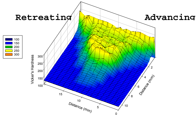
Figure 2.7b: Hardness variation in friction-stir processed NAB. Note large hardness increase in stir zone.
