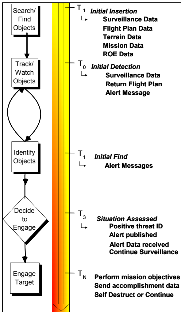
Figure 4: Possible “Cyber-Craft” Scenario
