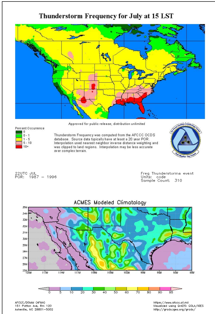
Figure 14. Thunderstorm probability plots for comparable times based on the Climo Atlas (top) and the ACMES model output (bottom).
