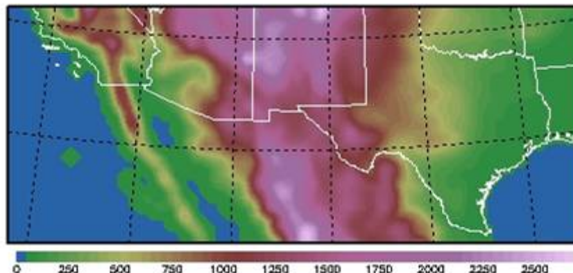
Figure 7. Terrain elevation in meters.
