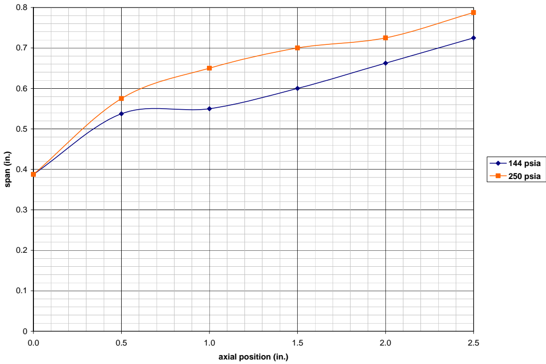
Figure 7: Maximum plume width profiles for baseline cases.
