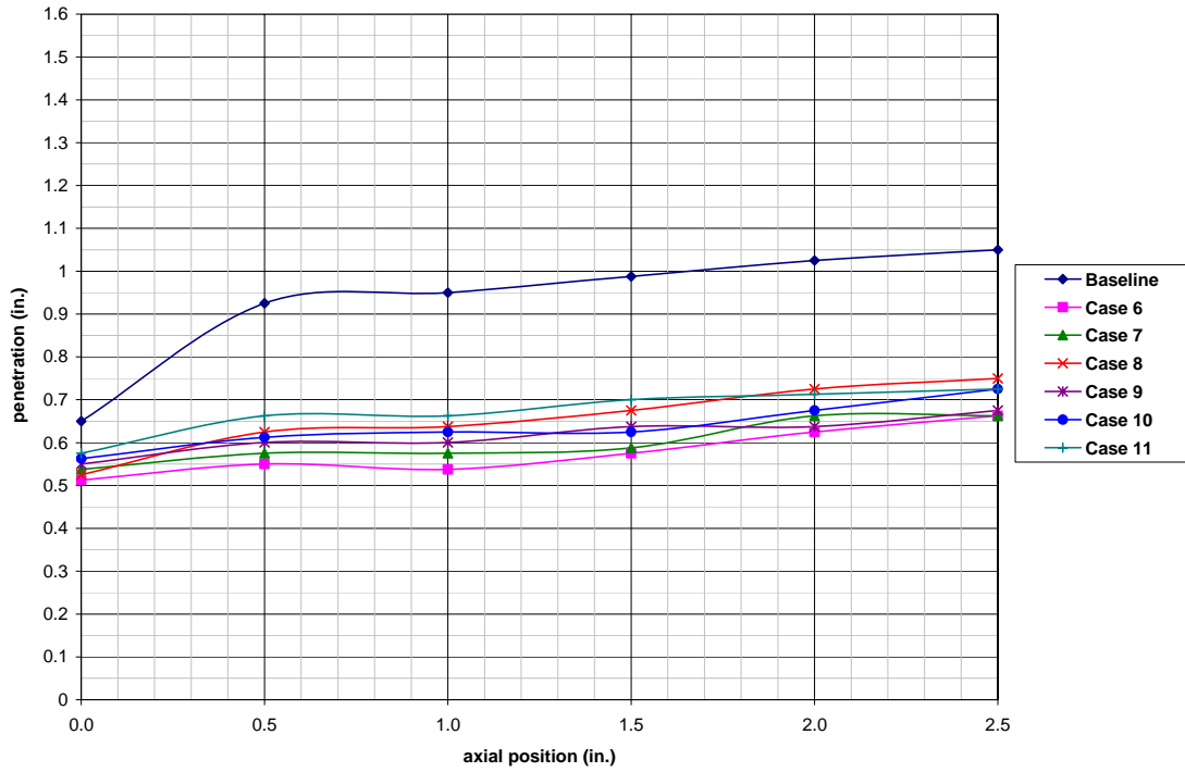
Figure 10: Transverse penetration profiles for cases with 2 active stages, P_{inj} = 144 psia
