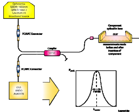
Figure 3. FBG LI performance measurement setup.
