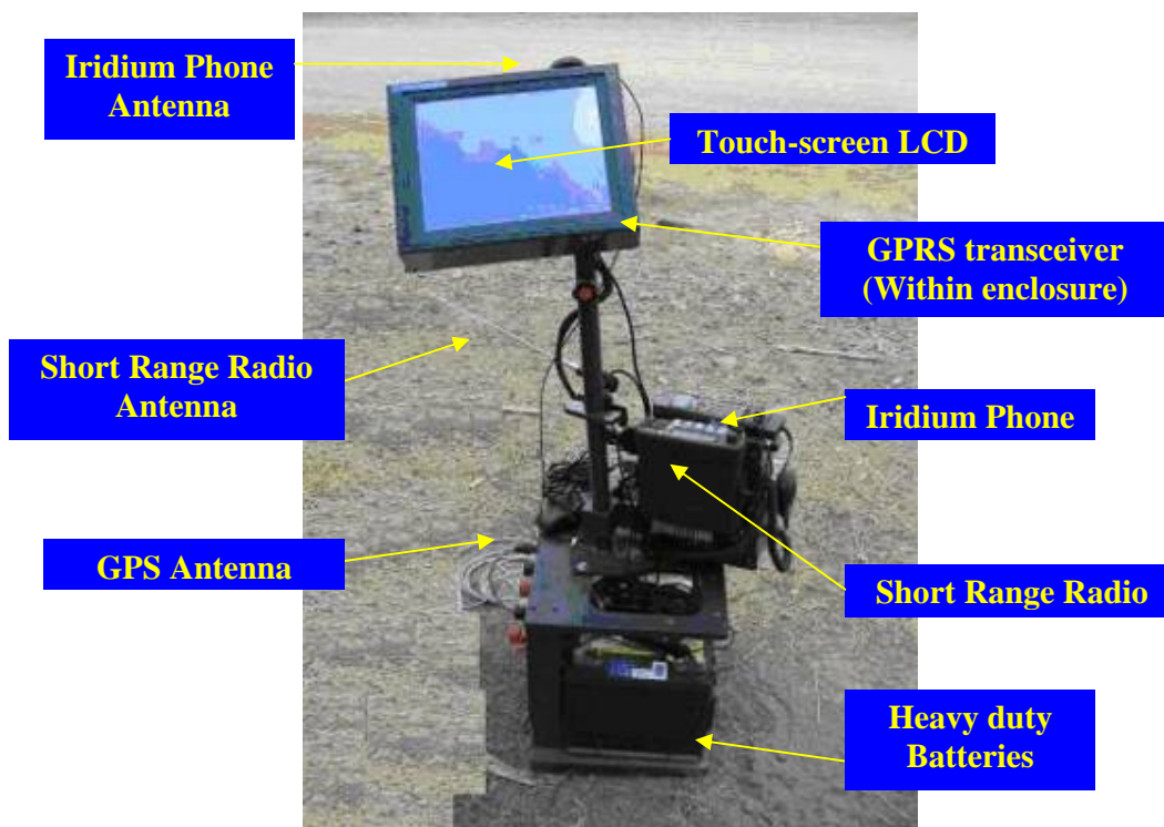
Figure 4: In-Vehicle-Unit (IVU)
