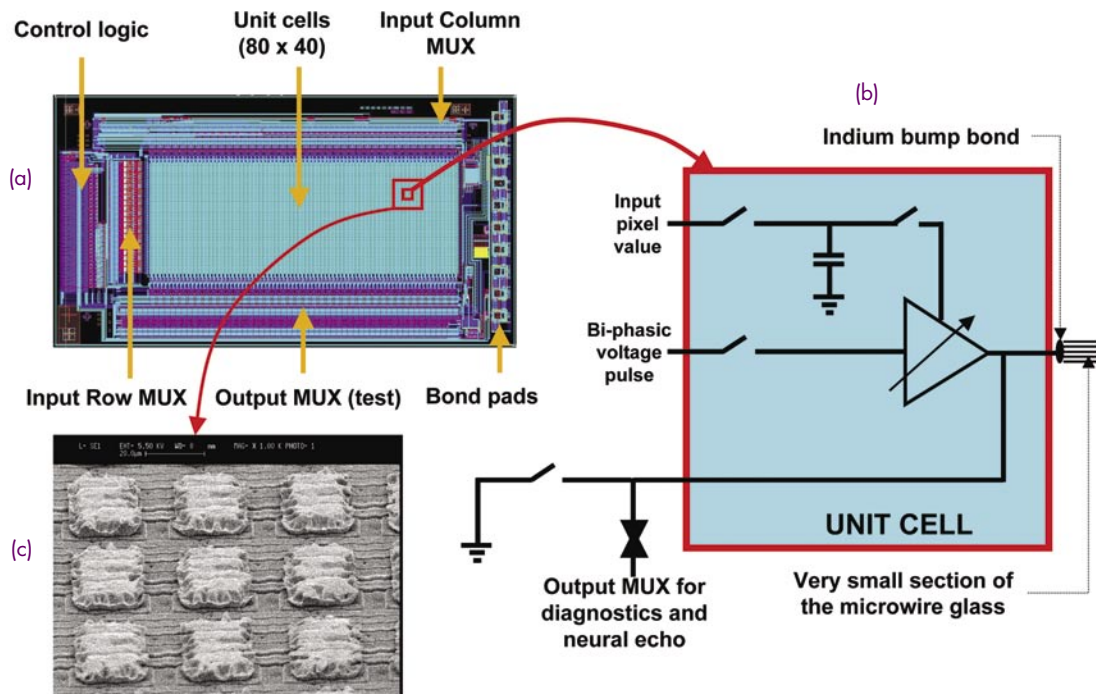
FIGURE 3 The microelectronic multiplexer floor plan is shown in (a) and a simplified schematic of the electronics in each unit cell (pixel) is shown in (b). Each unit cell has its own charge storage capacitor and a transconductance amplifier. The storage capacitors control the brightness of all 3,200 pixels within each frame. In (c), a scanning electron microscope (SEM) image of nine indium “bumps” is shown. There is one indium bump for each unit cell. Microwires on the flat side of the microwire glass will be pushed into all the bumps, connecting approximately 20 microwires to the output of each transconductance amplifier in the array. The opposite ends of those microwires will become the microelectrodes that send electrical stimulation into the retina.
