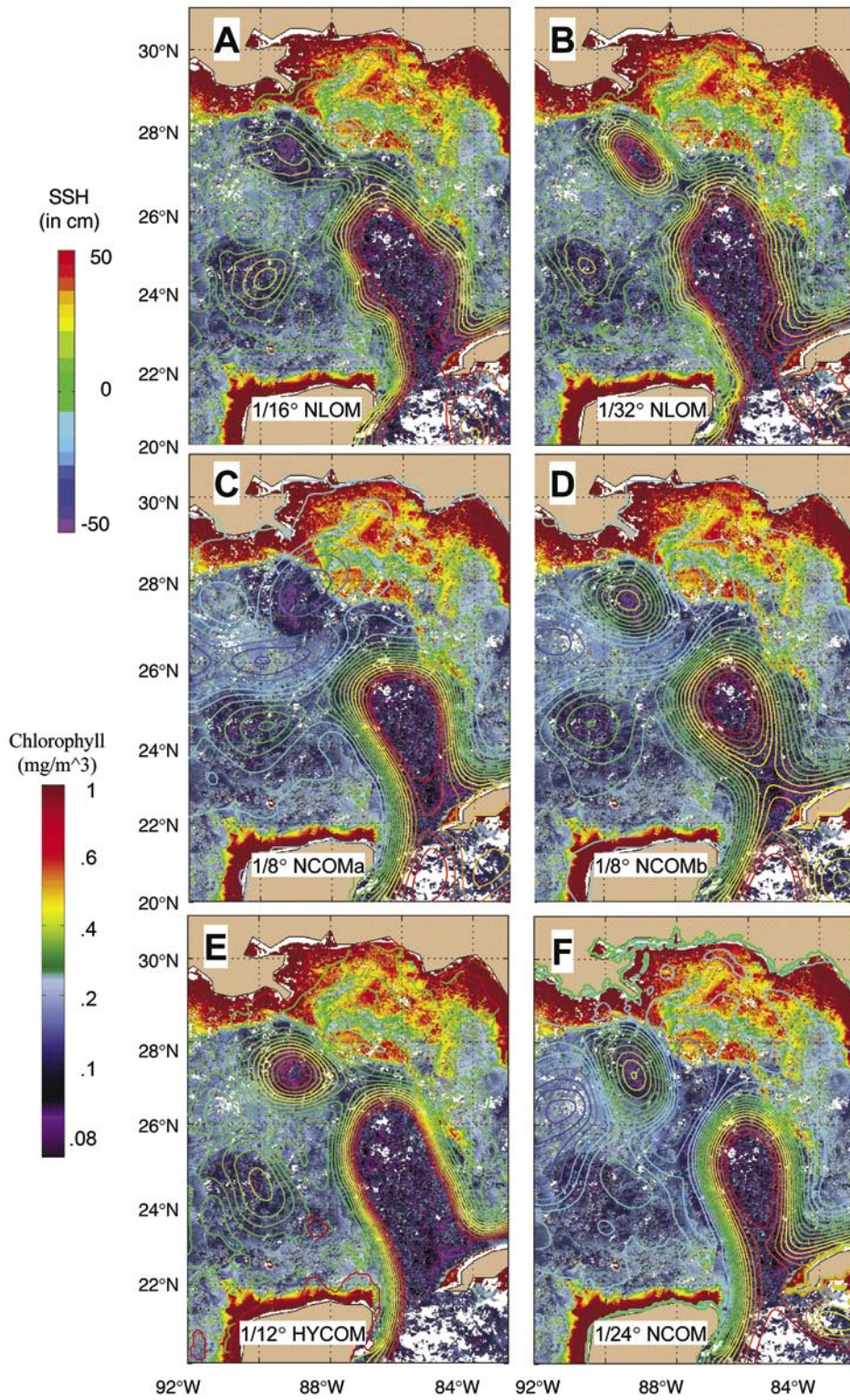
FIGURE 7 Nowcast SSH line contours from 6 ocean prediction systems or their variants on 28 August 2003 overlaid on ocean color imagery from SeaWiFS. Both the SeaWiFS imagery and the SSH contours are colored prismatically from low (violet) to high (red). The SeaWiFS chlorophyll concentration is the latest cloud-free pixel composite over 22-28 August 2003. SSH from the GFO and JASON-1 altimeters are used for assimilation. SSH contour interval is 5 cm, and contours >50 cm are omitted.
