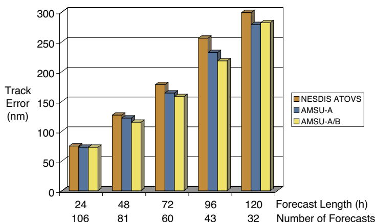
FIGURE 8 Comparison of the mean tropical cyclone track error vs forecast hour for the month of September 2003. Verification is against the postseason "best track." The numbers below the forecast length are the total number of forecast tracks for the month used in the comparison.
