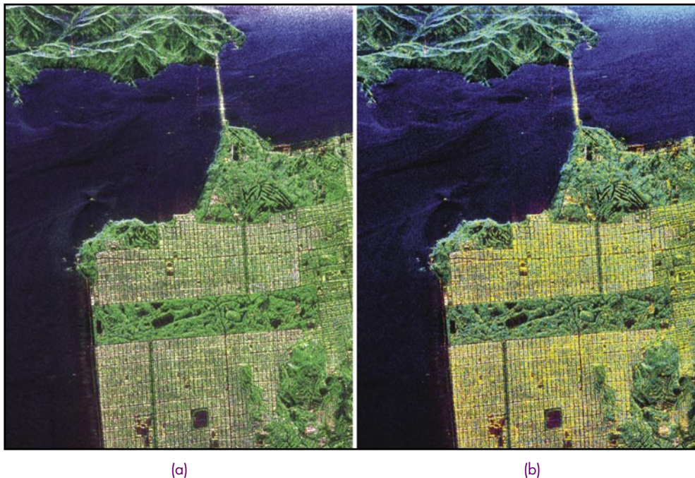
FIGURE 4 (a) NASA JPL POLSAR image of San Francisco displayed with |HH-VV| , |HV| , and |HH + VV| , for red, green and blue, respectively. (b) The Freeman/Durden decomposition using |P_{DB}| , |P_V| , and |P_S| for red, green, and blue.
