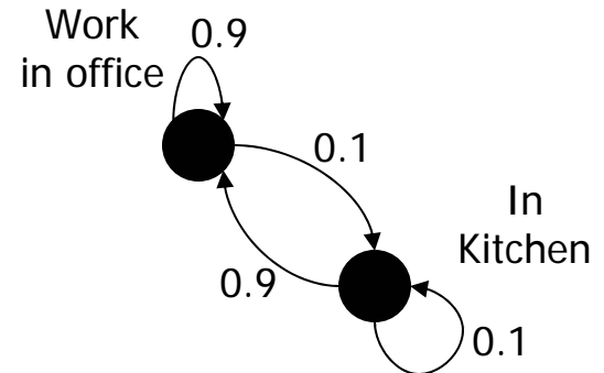
HMM-2
