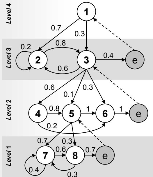
(a) Hierarchical HMM
