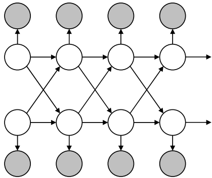
(a) Fully-coupled HMM
