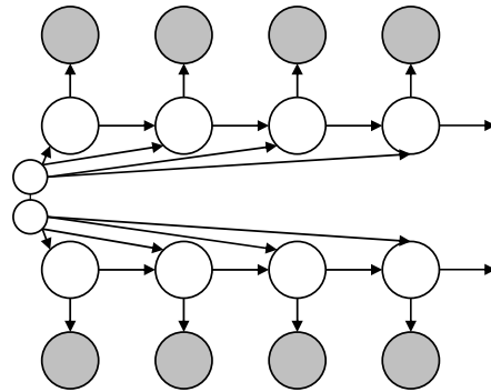
(b) Event-coupled HMM
