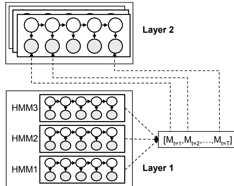
(b) Layered HMM
