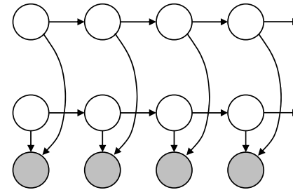
(c) Factorial HMM
