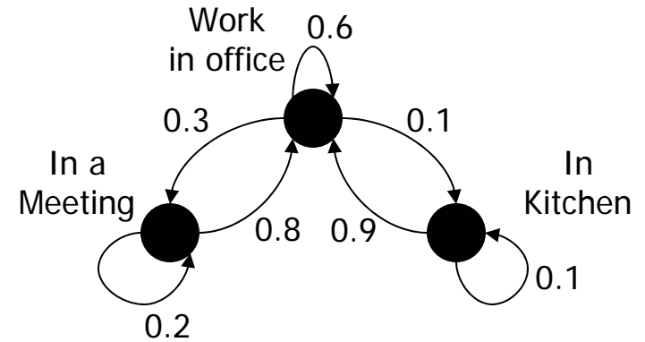
HMM-1
