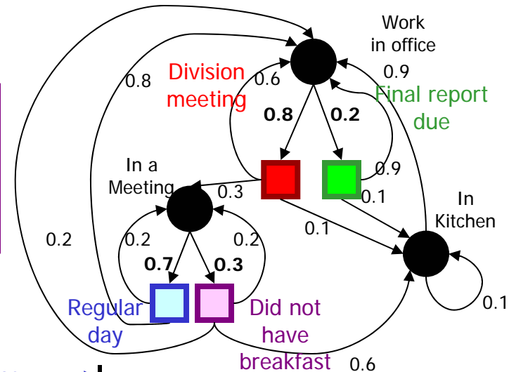
POMDP: effect of actions/decisions
