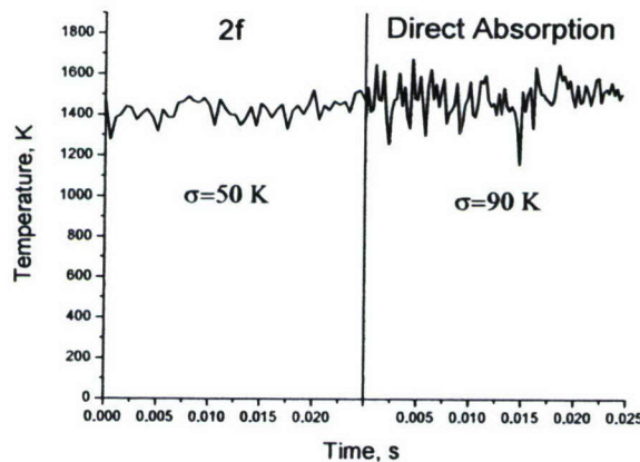
Figure 2.4.10. Comparison of measured temperature using direct absorption and WMS-2f with the 1392/1469 nm line pair. The direct absorption data is filtered from 4 kHz to 2 kHz to match the WMS-2f sampling rate. \phi = 1.02 .
