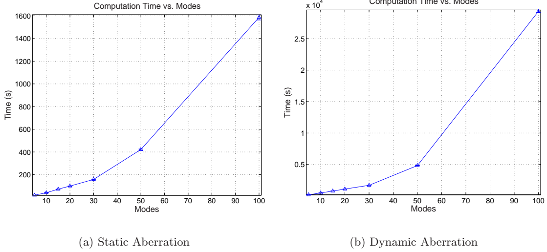
Figure 6.20: Computation time vs. modes for (a) static aberrations and (b) dynamic aberrations. Increasing the number of included modes initially improves MSE at the cost of a significant increase in computation time caused by the computational burden of including the extra modes in the system model.
