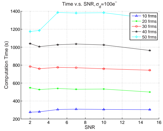
(b) \sigma_d = 100e^{-}
