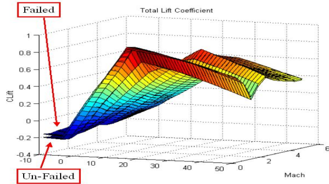
Figure 4. Lift Coefficient For Failed And Un-Failed Configurations.
