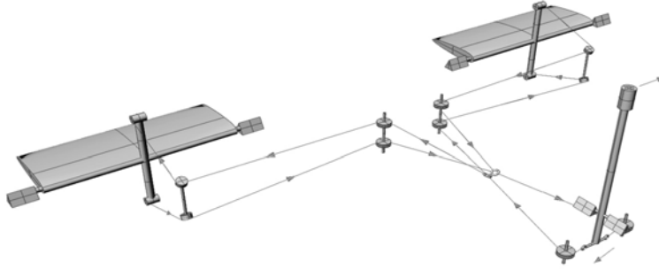
Figure 1. Mechanical ganging of ailerons on historical aircraft
