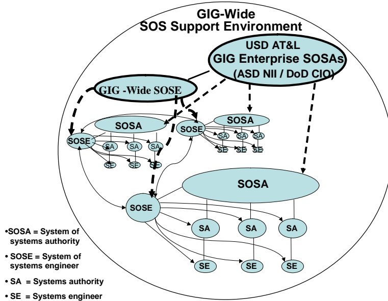
Figure 6: GIG Net-Centric System-of-Systems Engineering
