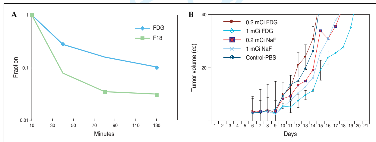
Figure 3. (A) After intratumoral injection, ^{18}\text{F} -FDG is retained in the tumors while ^{18}\text{F} -NaF exits rapidly. (B) The ability of ^{18}\text{F} positrons to suppress tumor growth after locoregional injection correlates with its retention in the tumors.
