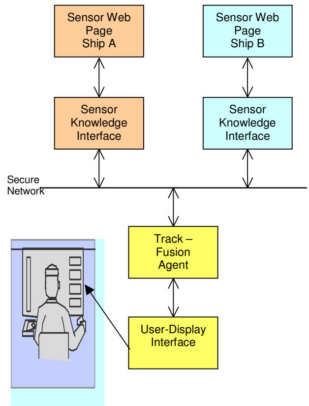
Figure 2. KMDT concept of operations, as shown in this agent - application functional diagram [8]
