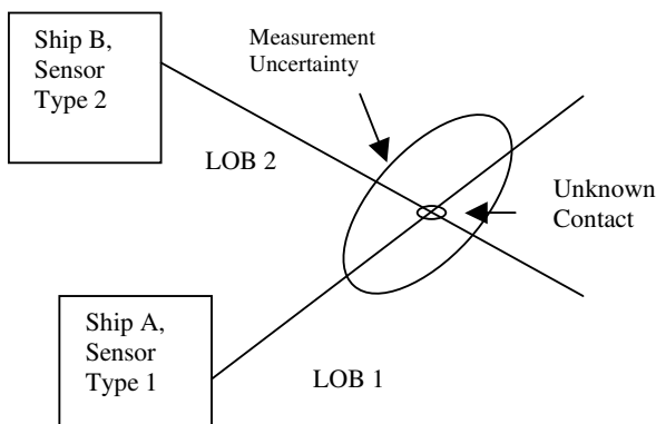
Figure 1. Platform detection geometry showing lines of bearing from ships A and B detecting an unknown contact with heterogeneous sensor types 1 and 2 [7], [8].
