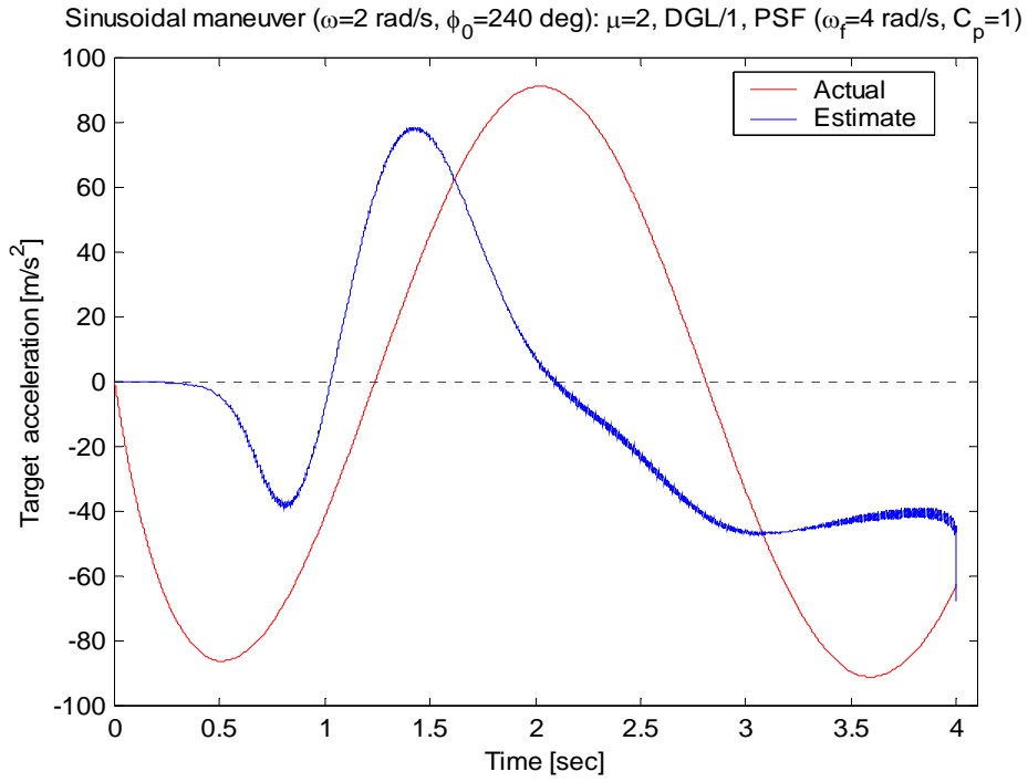
Fig. B.4. Estimation of target lateral acceleration with unmatched PSF
