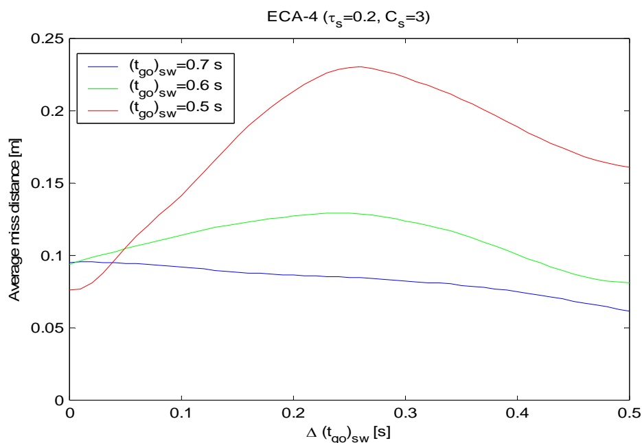
Fig. 6. Homing performance with “tuned” estimators
