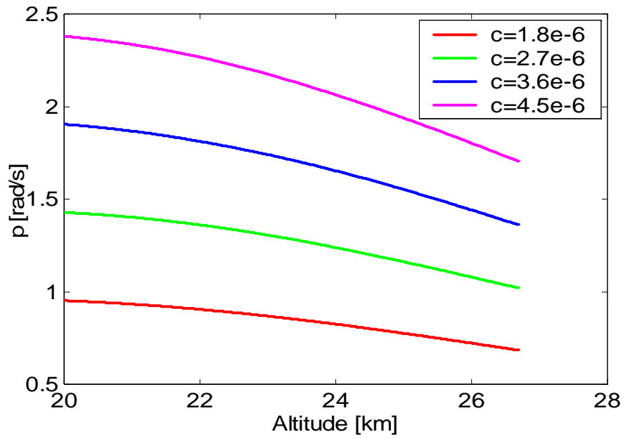
Fig. D.8. Nominal endgame roll rate profiles for h_{int} = 20 km
