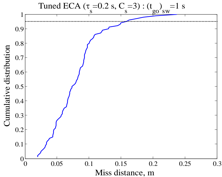
Fig. 8. Cumulative miss distance distribution of DGL/1 with a perfectly “tuned” estimator
