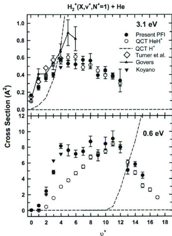
FIG. 9. PFI-PESICO measurements by Tang et al. (Ref. 49) (filled circles) of H_2^+(v^+, N^+=1) + He proton-transfer cross sections as a function of vibrational quantum number ( v^+ ) at two translational energies, E_T=0.6 and 3.1 eV. The PFI-PESICO errors bars represent statistical errors. The experimental results are compared with experimental results by Turner et al. (Ref. 8) (open diamonds), Govers and Guyon (Ref. 4) (upward pointing filled triangles), and Koyano and co-workers (Refs. 11 and 63) (downward pointing filled triangles). The measurements of Turner et al. are the averages of measurements at E_T=2 and 4 eV. QCT calculations by Tang et al. (Ref. 49) of the proton transfer (open circles) and dissociation (dashed lines) cross sections including zero-point energy restrictions are also shown.
