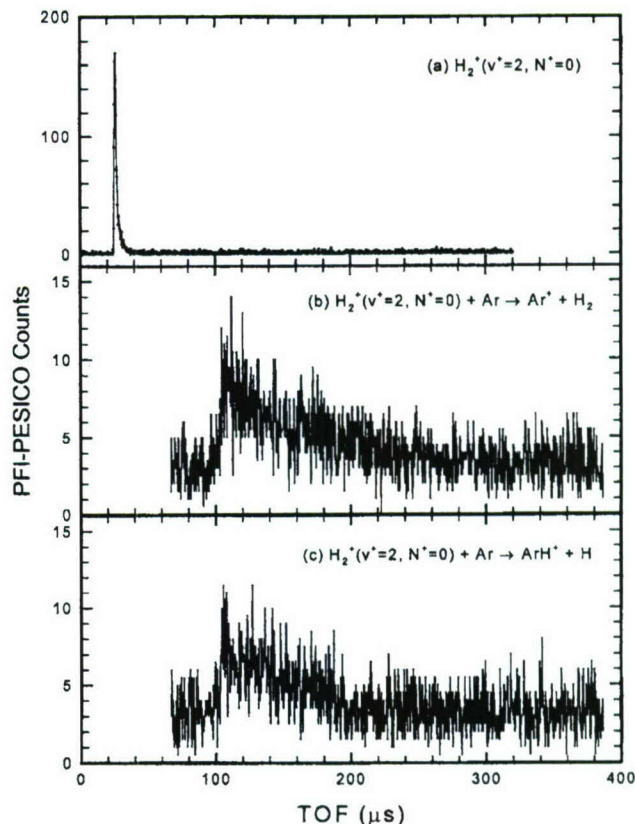
FIG. 3. TOF spectra of PFI-PESICO ions observed in \text{H}_2^+(v^+=2, N^+=0)+\text{Ar} collisions. (a) Primary ion PFI-PEPICO spectrum. (b) \text{Ar}^+ product ion PFI-PESICO spectrum. (c) \text{ArH}^+ product ion PFI-PESICO spectrum. Taken from Ref. 46.
