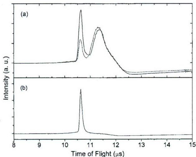
FIG. 11. (a) TOF spectrum showing the \text{NO}^+ PFI-PI and prompt background ion peaks (observed using an oscilloscope). The spectra were obtained with the VUV set at the IE[ \text{NO} \rightarrow \text{NO}^+(v^+=1) ]. The solid and dot curves correspond to the measurements with and without the ringing scrambling electric field, respectively. (b) TOF spectrum showing the \text{NO}^+ PFI-PI peak after the prompt \text{NO}^+ background peak was blocked by a pulsed electric field applied to the lower repeller plate. Taken from Refs. 131 and 137.
