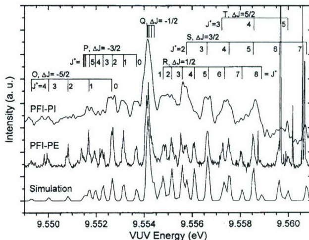
FIG. 12. Comparison of the rotationally resolved PFI-PE spectrum (middle), the PFI-PI spectrum (upper), and the simulated (bottom) spectra for \text{NO}^+(X, v^+=1, J^+) \leftarrow \text{NO}(X, v''=0, J'') . The spectral simulation gives a rotational temperature of 50 \text{ K} for \text{NO} . Taken from Refs. 131 and 137.
