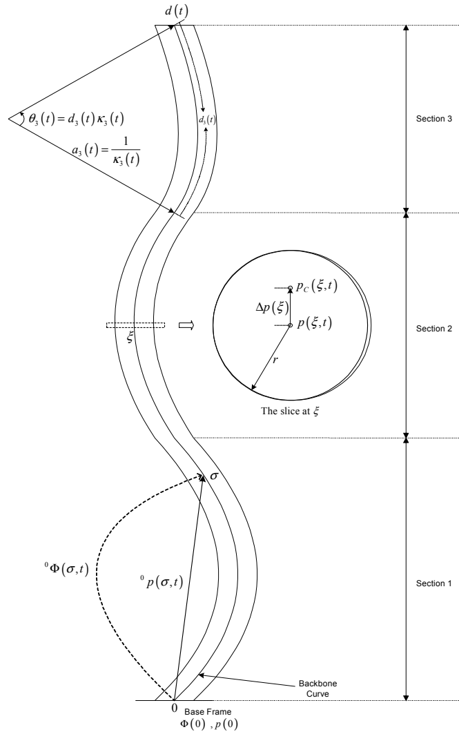
Figure 2: Geometry of a 3-Link Extensible Robot Manipulator
