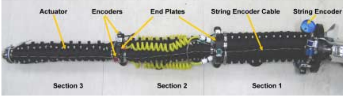
Figure 1: Octarm Continuum Robot (version 5.2) in Clemson University Mechatronics Laboratory
