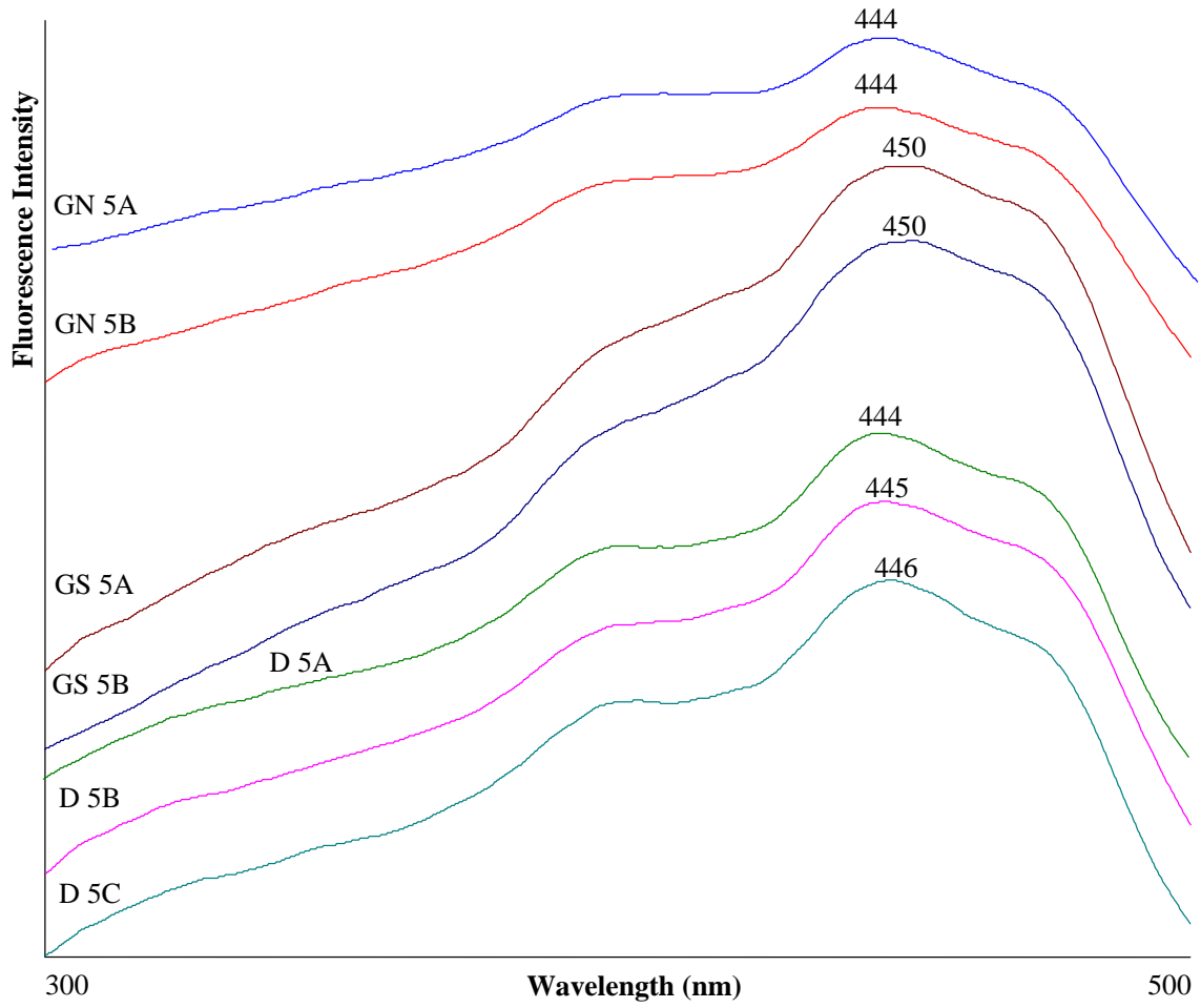
Figure 15. Excitation fluorescence spectra of the humic acids extracted with 0.5 M NaOH from greenhouse soils where the germplasm line SERDP-select of Siberian wheatgrass was grown.
