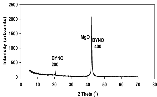
Fig. 1. X-ray diffraction pattern of BYNO film deposited on MgO (100) substrate. MgO (200) peak and BYNO (400) peak are overlapped on each other.
