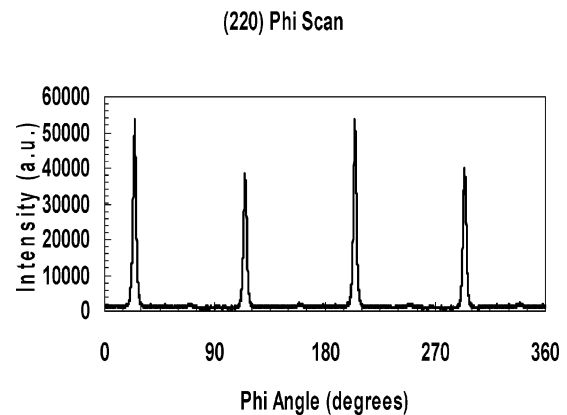
Fig. 3. X-ray Phi scan of (220) reflection of BYNO film deposited on IBAD MgO substrate.
