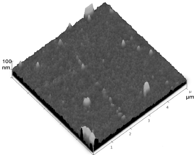
Fig. 4. Atomic Force Microscope image of BYNO film surface ( 5 \mu\text{m} \times 5 \mu\text{m} area) deposited on IBAD MgO substrate. X-Scale is 1 \mu\text{m}/\text{unit} division and Z-Scale is 50 \text{ nm}/\text{unit} division.
