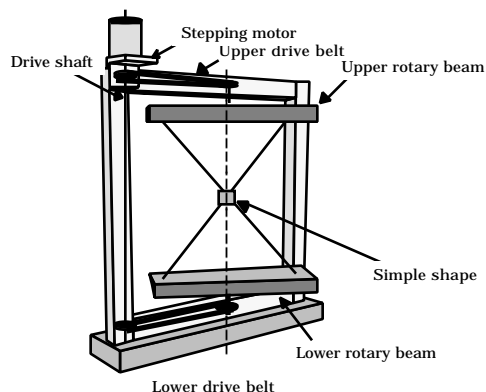
Figure 3. Free-space 360° sling mount used for small, low-RCS targets.
