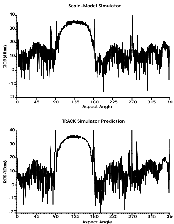
Figure 9. Comparison between computer predictions and modeled measurements of the complex target simulator.
