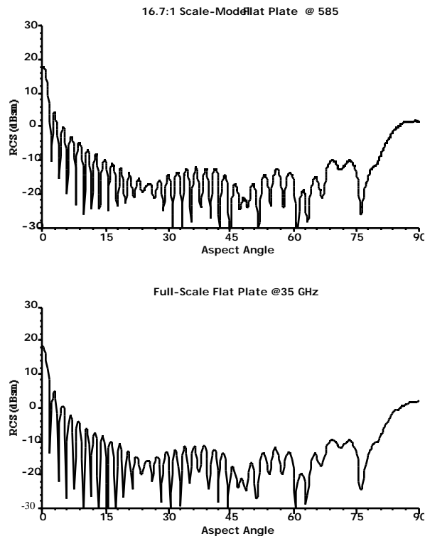
Figure 6. Comparison between full-scale and model measurements of a flat plate.
