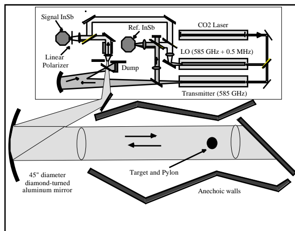
Figure 1. Diagram of 585 GHz transceiver and compact range.
