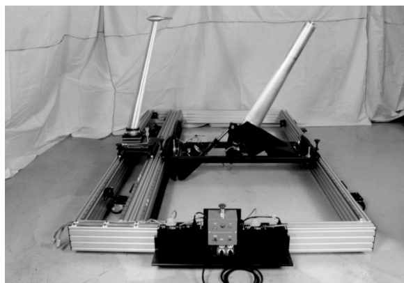
Figure 4. Side view of the free-space calibration (left) and target (right) pylons on translation base.
