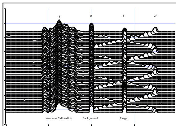
Figure 2. Waterfall plot showing a sequence of spectra processed from the target modulation. Each trace represents a different aspect angle.
