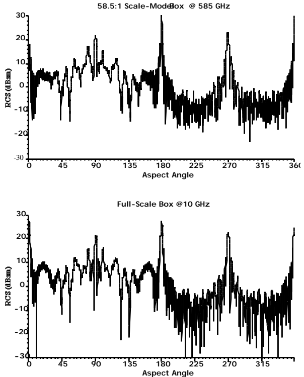
Figure 7. Comparison of full-scale and modeled rectangular box with cavities.
