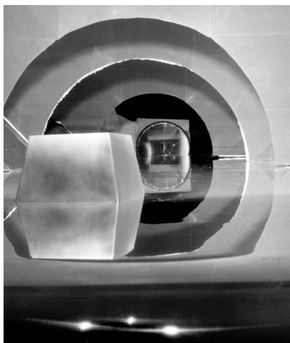
Figure 5. Truncated pyramid and its image on the submillimeter range ground plane looking towards the 45" antenna mirror.
