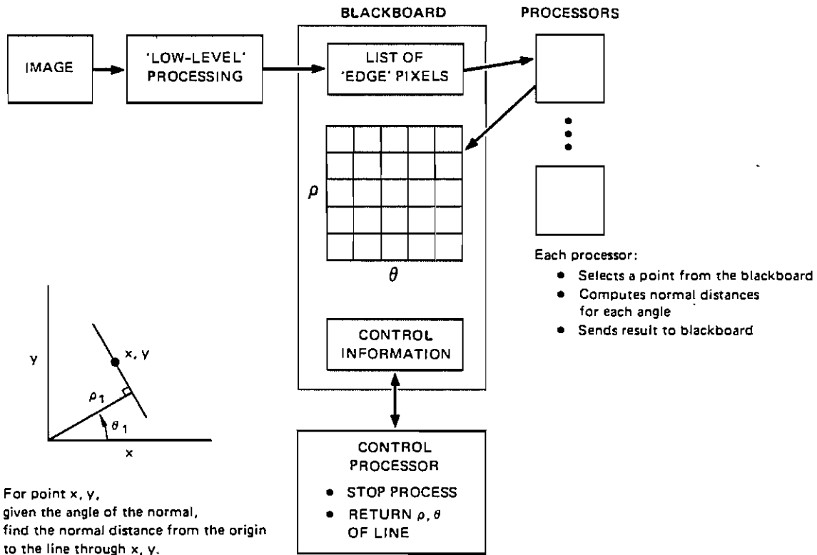
FIGURE 2 HOUGH APPROACH
