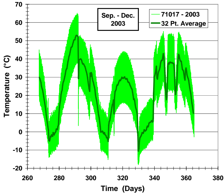
Figure 12 Time-temperature history of MISSE-1 & -2 data loggers
