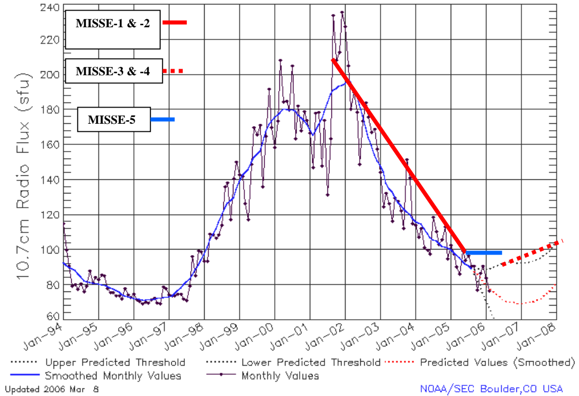
Figure 3 Variation in solar activity over a solar cycle, as represented by 10.7 cm flux ground measurements
