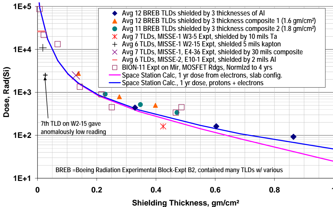
Figure 21 Dose from TLDs on MISSE-1 and MISSE-2 as Function of the Thickness of Aluminum
