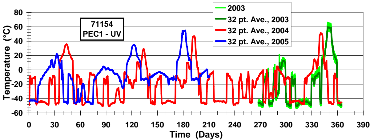
Figure 16 MISSE-1 UV-side, Average temperatures for datalogger 71154
