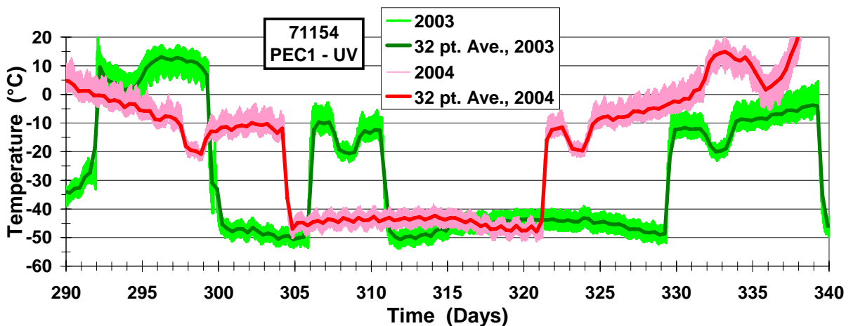
Figure 19 Temperature extremes recorded on datalogger 71154, MISSE-1 wake side
