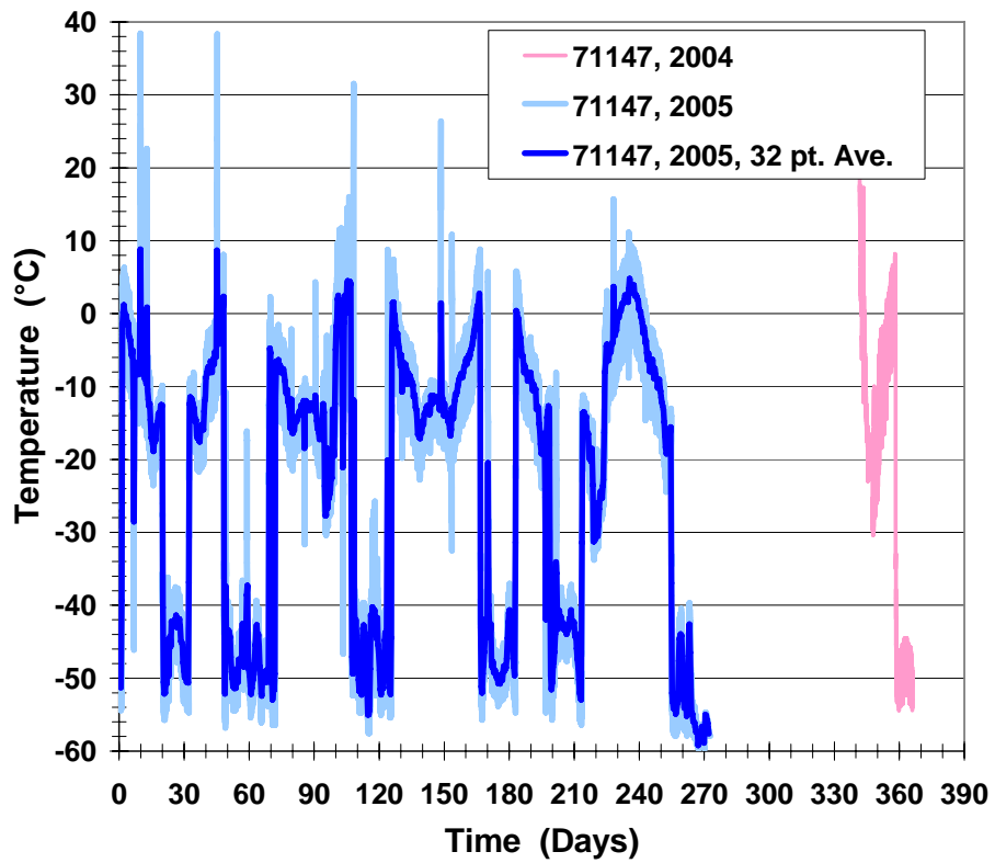
Figure 15 Average temperatures for datalogger 71147
