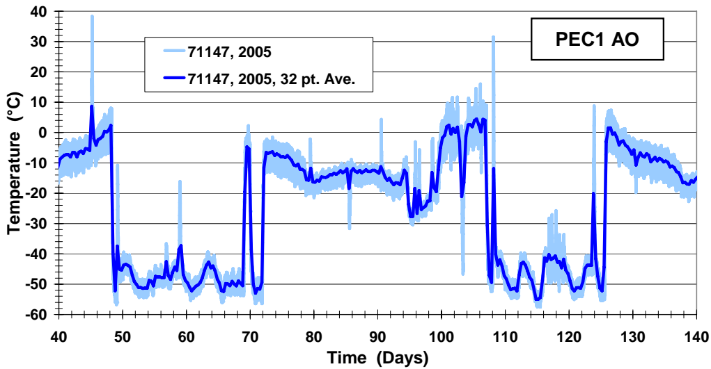
Figure 18 Temperature extremes recorded on datalogger 71147, MISSE-1 ram side
