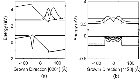
Figure 5. The remarkably high internal piezoelectric fields in wurtzite GaN/AlGaIn structures distort the band-edge potential in quantum wells, as shown in (a), leading to a poor overlap of carrier wavefunctions. When grown along the [11\bar{2}0] direction the piezoelectric fields are along the plane, leading to better characteristics for quantum well lasers. Strain, piezoelectric effects, and inversion asymmetry effects have been included in the calculations (after [19]). Figure reproduced with permission from Elsevier).
