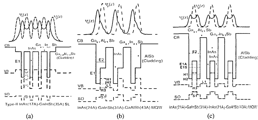
Figure 1. (a) The type-II heterostructure of InAs/GaInSb leads to localization of wavefunctions in different layers. This is ameliorated partially by introducing a step potential as in (b). The structure, shown in (c), provides a substantially improved overlap (figure adapted from [4, 26]; with permission from Elsevier).
