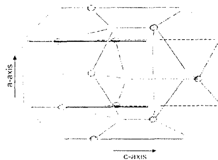
Figure 2: The Wurtzite heterostructures grown on the R-plane, i.e., with layers stacked along the a -axis, show no spontaneous polarization. Thus quantum wells grown along this direction will not have their bandedge profiles distorted by any polarization fields.
