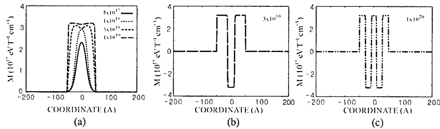
Figure 4. The magnetization due to Mn spin alignment in a 100 Å GaMnAs quantum well is shown. In (a), the alteration of magnetization with increasing hole concentrations from 5 \times 10^{17} \text{ cm}^{-3} – 10^{19} \text{ cm}^{-3} is shown. With further increases in hole concentration, (b) and (c), the magnetization oscillates in orientation across the quantum well. This is due to the occupied energy levels and the corresponding wavefunctions for holes in the self-consistent potential (after [24]).
