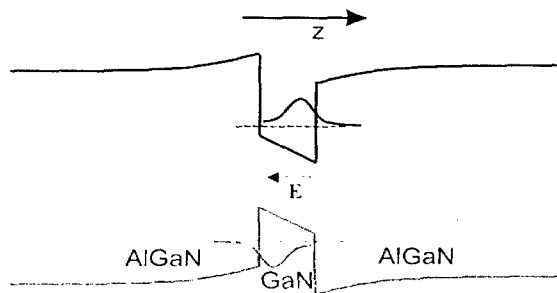
Figure 1: A schematic of the band bending in layered structures grown along the c -axis, due to spontaneous polarization and piezo-electric fields. The distorted bandedges lead to poor wavefunction overlap.
