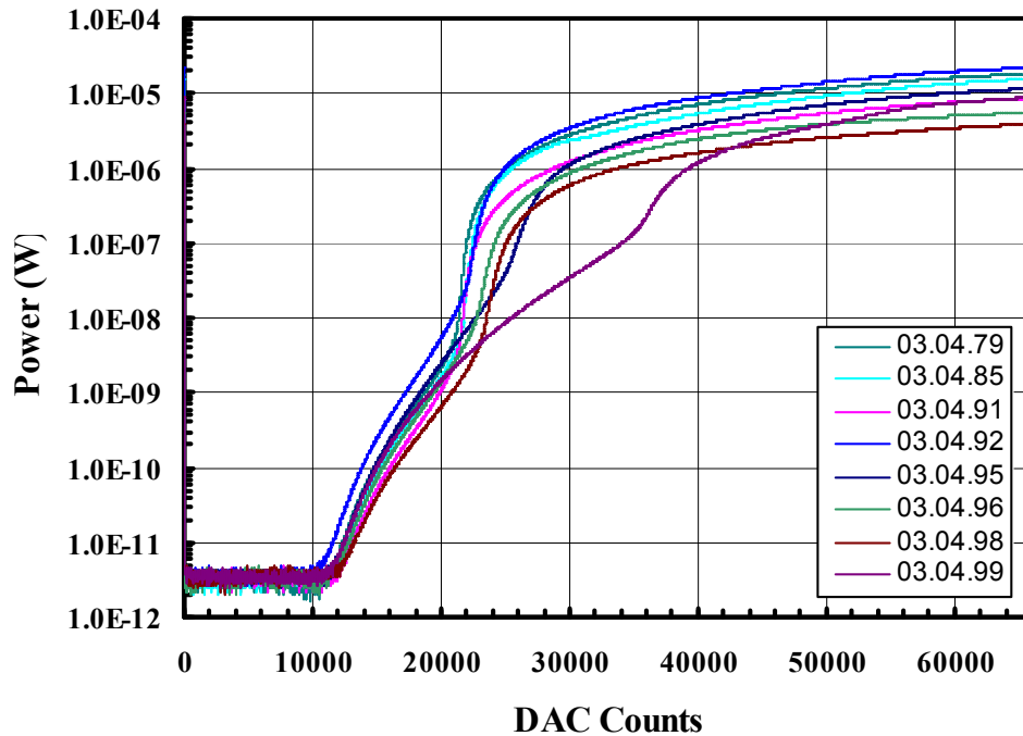
Figure 10. Laser output power as a function of DAC count for the lasers employed in the multi-channel system
