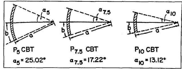
Fig. 1. Geometry of P 5 CBT (left), P 7.5 CBT (center), and P 10 CBT (right).
