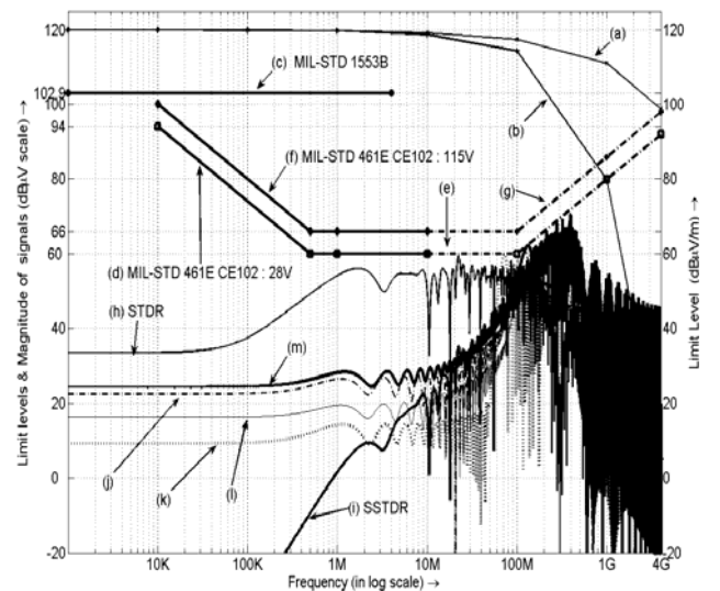
Fig. 1. EMI Standards, attenuation curves, and spectral content of test signals (a) Attenuation for 100' of RG58 coaxial line, (b) Attenuation for 100' of two wire line, (c) MIL-STD 1553B, (d) MIL-STD 461E CE102 for 28V DC lines, (e) MIL-STD 461E RE102 assumed continuous with the CE102 standard, (f) MIL-STD 461E CE102 for
