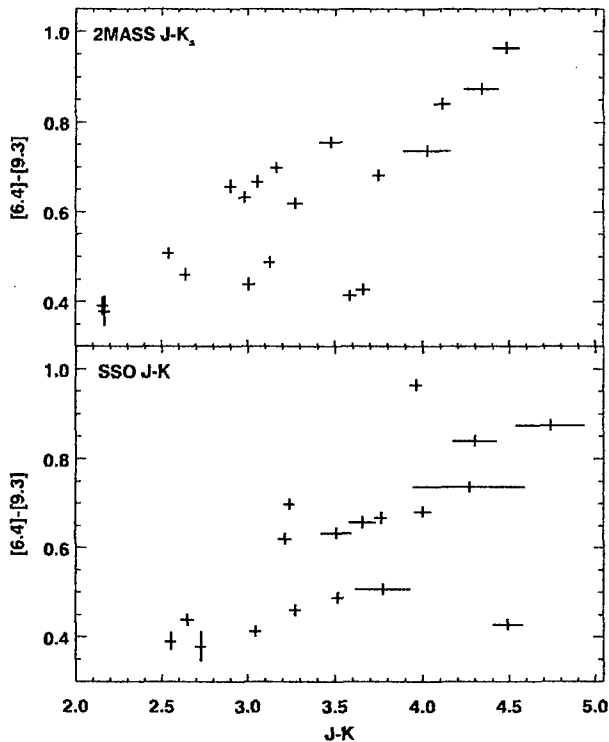
FIG. 6.—The [6.4] - [9.3] colors extracted from the spectra, plotted as a function of J - K color. The top panel plots the 2MASS J - K color, and the bottom panel plots the SSO J - K color. In both cases, the [6.4] - [9.3] color correlates reasonably well with the near-infrared color. The overall shift between the two J - K colors results from the shift in the position of the J and K bands between the two systems. The two most notable outliers at J - K , \sim 3.6 and [6.4] - [9.3] \sim 0.4 are MSX SMC 066 and 200. MSX SMC 200 is the only outlier when looking at SSO J - K color.
