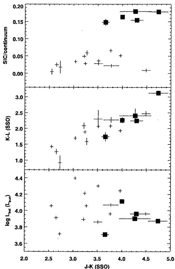
FIG. 12.—Strength of the SiC dust emission as a function of J - K color (top), our sample plotted on a JKL color-color diagram (middle), and bolometric luminosity vs. J - K color (bottom). The strong SiC sources are plotted with boxes. The photometry is from SSO, although it should be noted that the dependence on 2MASS J - K_s colors is similar. The strong SiC sources tend to be among the redder sources in our sample, especially at J - K . Section 2.4 explains how we estimated the bolometric luminosity. The strong SiC sources are not among the brightest sources in the sample. [See the electronic edition of the Journal for a color version of this figure.]
