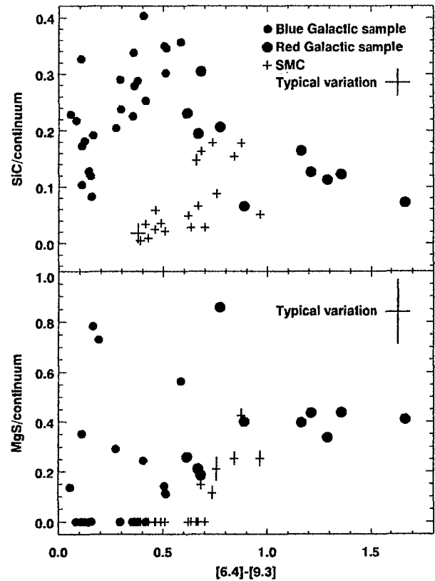
FIG. 8.—Strength of the dust emission features from SiC at 11.3 \mu m and MgS at \sim 30 \mu m as a function of [6.4] - [9.3] color. Symbols are as in Fig. 7. The SMC sample tends to show weaker dust emission than the Galactic sample. [See the electronic edition of the Journal for a color version of this figure.]
