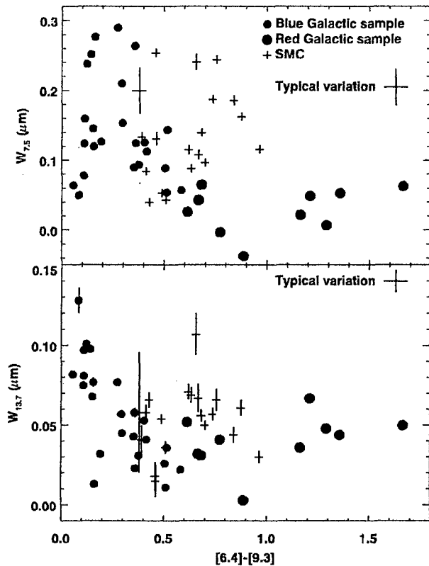
FIG. 7.—Equivalent widths of the C_2H_2 bands at 7.5 and 13.7 \mu m as a function of [6.4] - [9.3] color for both the SMC sample (plus signs) and the SWS Galactic sample (circles). The redder sources in the SMC sample show stronger absorption bands than their counterparts in the Galaxy. The black cross labeled “typical variation” reflects the expected impact on the data from the variability of the star, based on an analysis of those sources observed multiple times by the SWS. [See the electronic edition of the Journal for a color version of this figure.]
