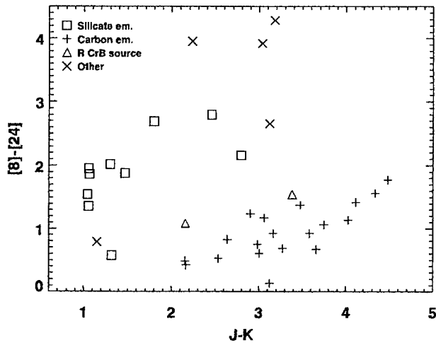
FIG. 1.—Color-color plot of the SMC sample. Plotting mid-infrared colors vs. near-infrared colors separates the various dust compositions clearly. This example uses 2MASS colors on the horizontal axis and colors derived from our IRS spectra using the bandpasses for the IRAC 8\ \mu\text{m} and MIPS 24\ \mu\text{m} filters on the Spitzer Space Telescope . The carbon-rich dust sources fall along a clear sequence that is red in J - K but blue in [8] - [24] compared to the oxygen-rich sources. [See the electronic edition of the Journal for a color version of this figure.]
