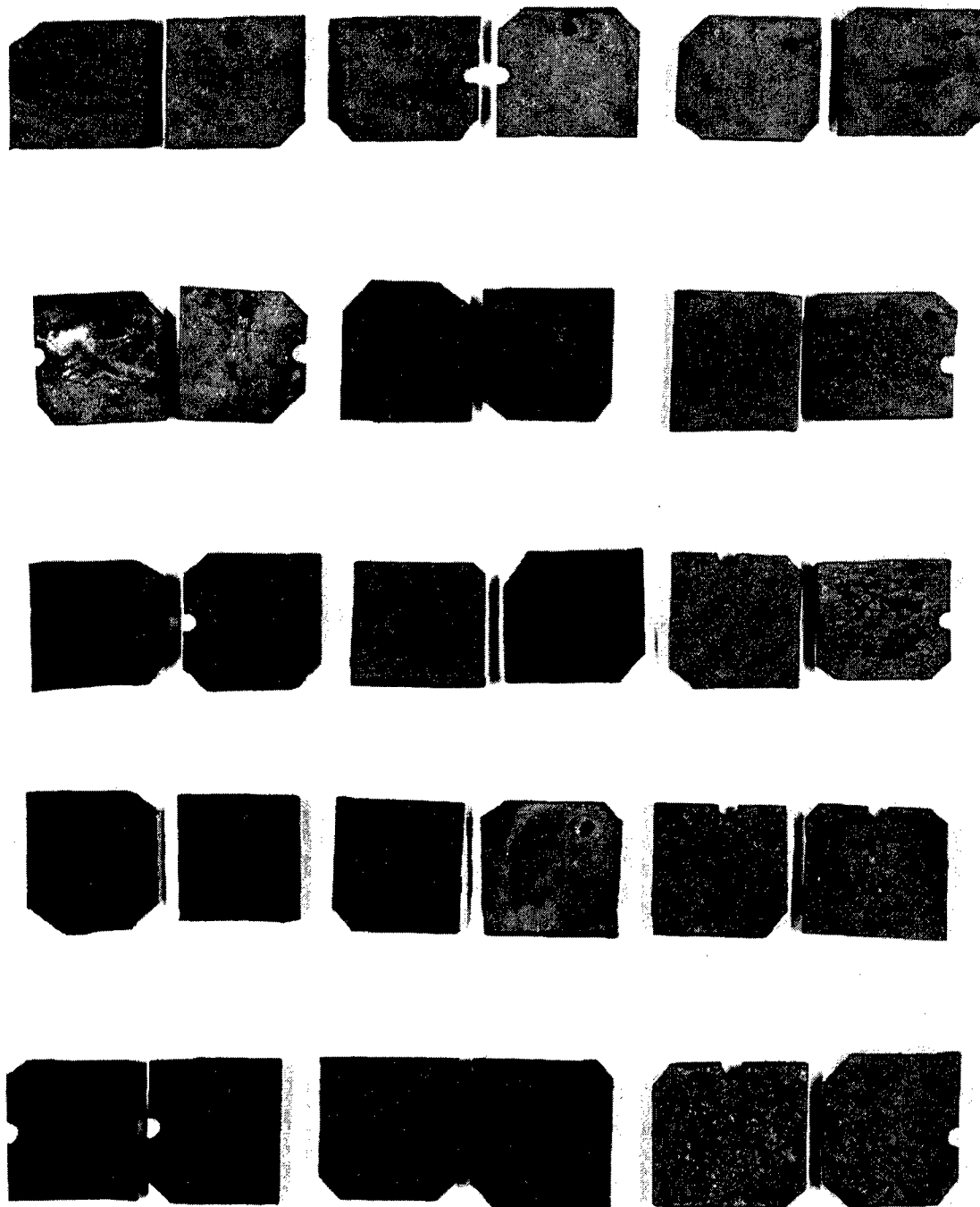
Figure 34. Cleaned Test Specimens after Exposure to 20% NaMnO 4 at Three Different Temperatures. The top panel is the test specimens after seven days of exposure, the next panel down is after 14 days, the third panel down is after 30 days, the fourth panel down is after 60 days, and the bottom panel is after 90 days. In all cases, the left two specimens were exposed at 60 °C, the middle two specimens were exposed at 80 °C, and the right two specimens were exposed at 100 °C.
