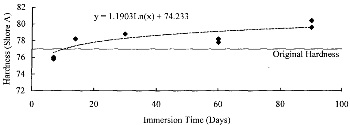
Figure 32. Changes in EPDM over Time when Immersed in 20 wt% NaMnO 4 Solution at 80 °C. The upper panel is the percent change in mass relative to the initial mass, the middle panel is the percent change in volume relative to the initial volume, and the lower panel is the change in hardness. The hardness values are averages of five readings from each test specimen.
