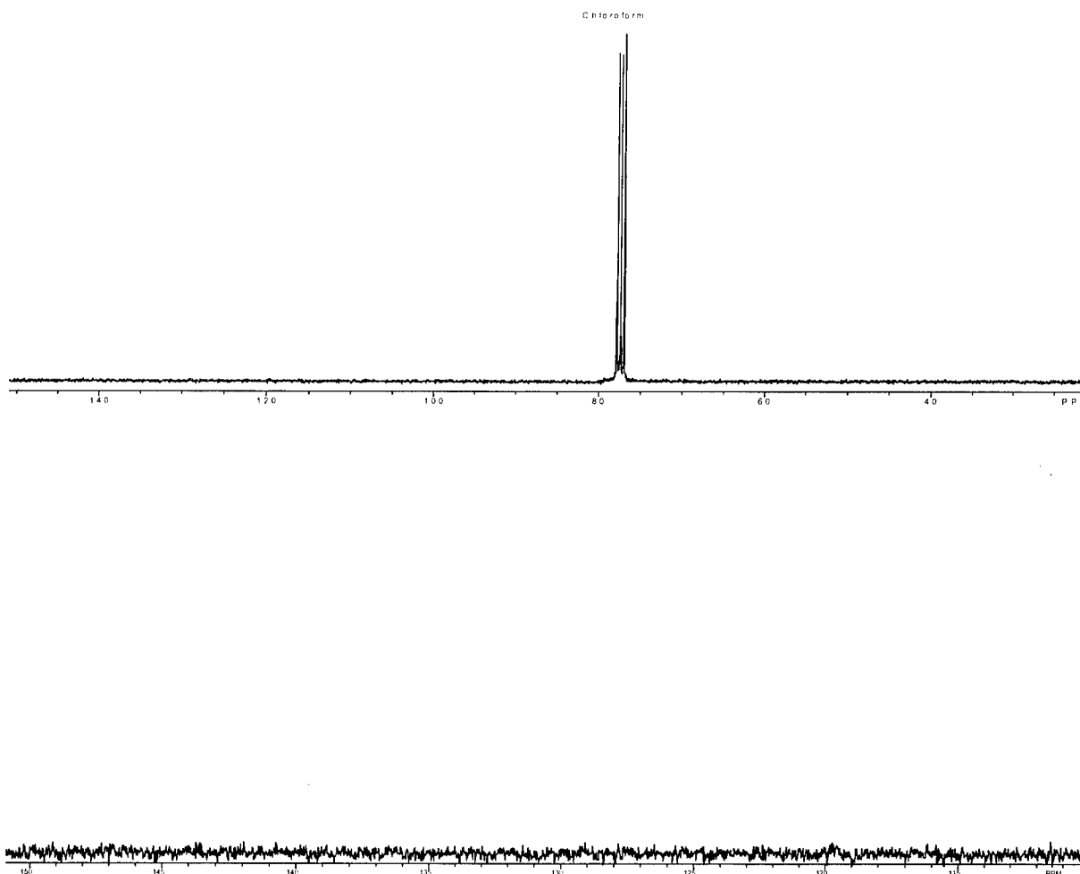
Figure 40. Example 13 C-NMR Spectra Obtained from the Analysis of the Isolated Sludge Solids from EDS Run Two. The upper panel is the full spectrum, and the lower panel is the spectrum zoomed into the chloro-vinyl shift region.
