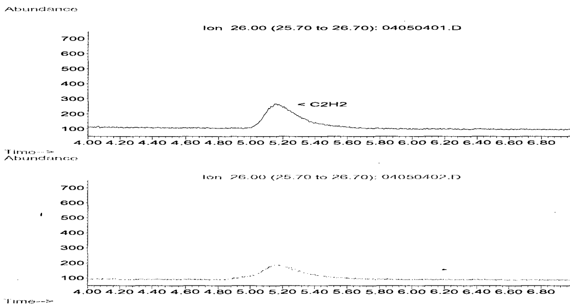
Figure 30. Comparison of the Headspace Gases Above a 20 wt% \text{NaMnO}_4 Reagent Blank (upper panel) and a Lewisite/Permanganate Reaction (bottom panel). The data was acquired by GC/MSD-EI, in SIM mode. The samples were both obtained after 15 min at 60 °C. The scales have been zoomed in to see the acetylene region of the chromatogram.
