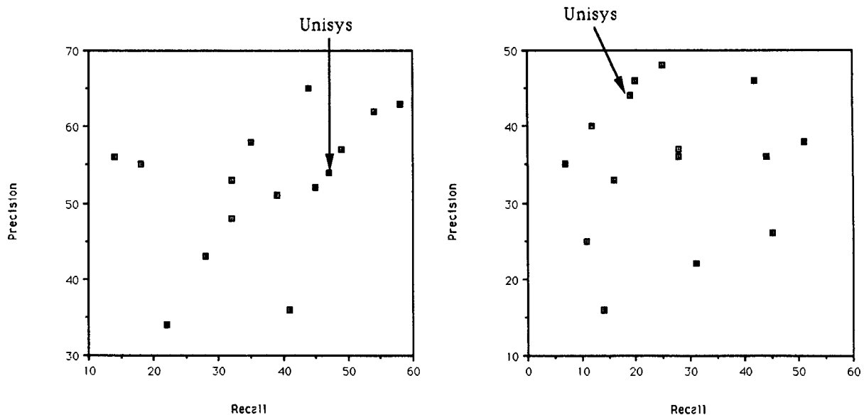
Figure 2: The scatter plot on the left indicates the relative performance of the Unisys MUC-3 system without taking into consideration false negative and false positive hits (the MATCHED-ONLY score). The scatter plot on the right indicates the relative performance of the Unisys MUC-3 system when taking into consideration both false negative and false positive hits (the ALL-TEMPLATES score).
