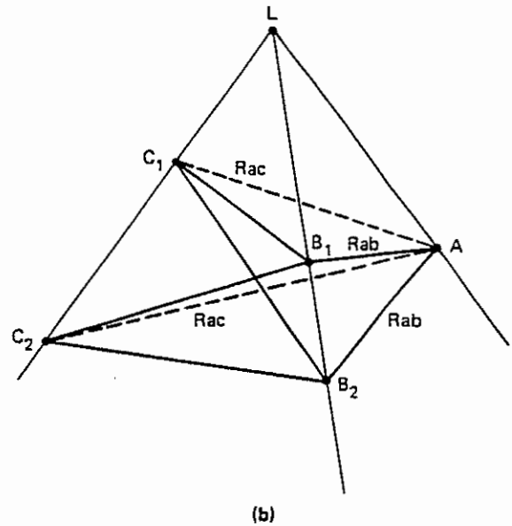
FIGURE 8 GEOMETRY FOR AN ITERATIVE SOLUTION TO THE P3P PROBLEM
