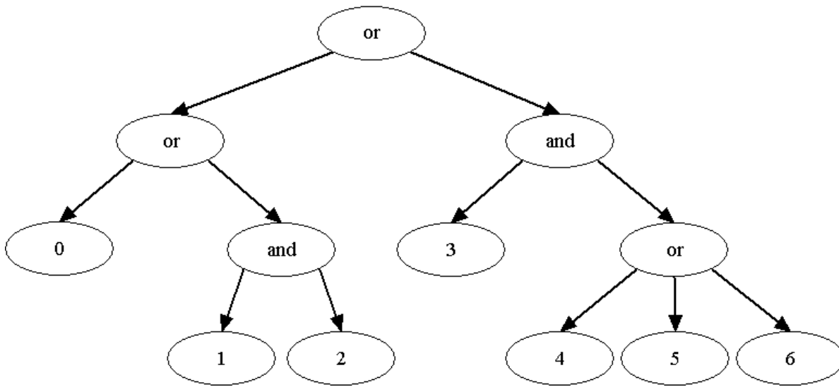
Figure 7. Fault Tree for Hazard h0
