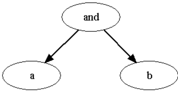
Figure 4. AND probability relationship
