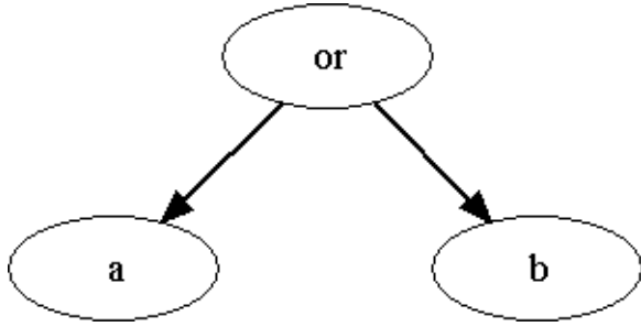
Figure 5. OR probability relationship
