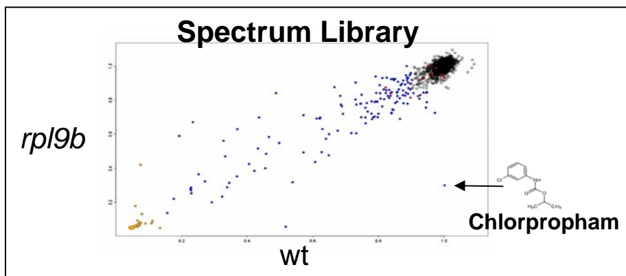
Figure 2. Spectrum Library differential screen against rpl9b \Delta . Wildtype (wt) or mutant ( rpl9b \Delta ) cells were screened against the Spectrum small molecule library at 20 \mu M concentration. Replicates are plotted on the corresponding axes. Activity is reported as normalized residual absorbance compared with DMSO controls. Individual compounds are represented by circles. Bioactive compounds ( Z > 4 ) are colored blue and cytotoxic compounds ( < 2SD from cycloheximide control) are shown in orange. Inactive compounds are open circles and red circles did not replicate within 20%. The molecule with greatest differential activity is denoted by an arrow.
