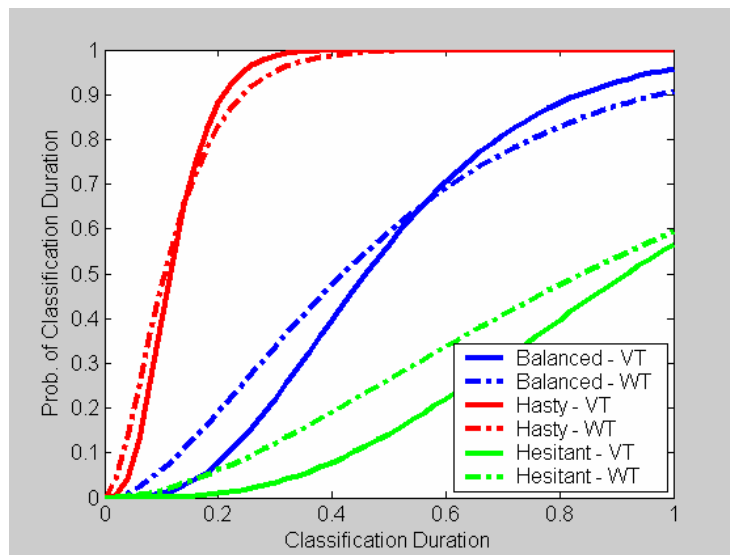
Figure 4. Cumulative probability distribution of the classification duration within a classification window of length 1 for Expert operators with different speeds. When classifying target of the same type, Hasty operator is always more likely to decide than Balanced operator, and Balanced operator is always more likely to decide than Hesitant operator.
