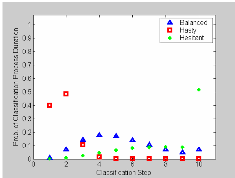
Figure 7. Probability of classification process for the suggested operators in ten time-intervals model (time intervals are of length T/10 ).
