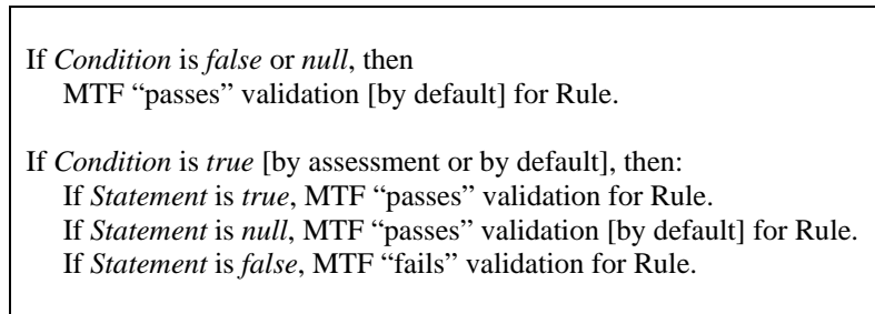
Figure 1. Rule evaluation logic
