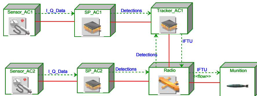
Figure 2. Subsystem Information Flows
