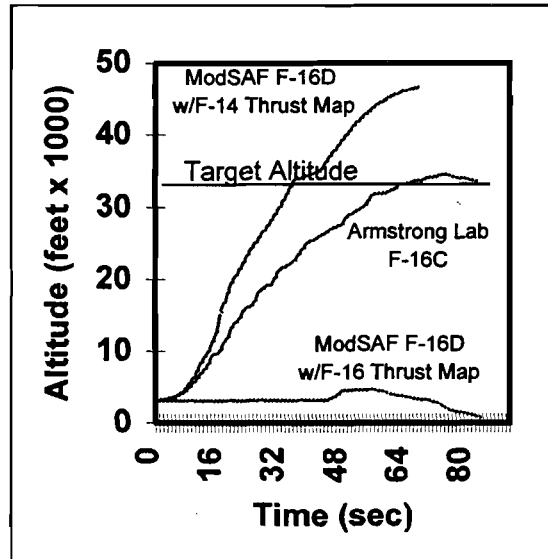
Figure 2 F-16 Climb Performance Comparison
