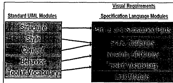
Figure 3. UIML to Visual Requirements Language Mapping
