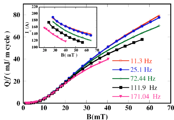
FIG. 1. (Color online) Energy loss in the uniform sample per unit length, per cycle ( Q/f ) at five different frequencies, from 11.3 to 171 Hz, plotted vs amplitude of the applied magnetic field. The inset shows the bulk average critical current obtained from the loss data by inverting Eq. (1).
