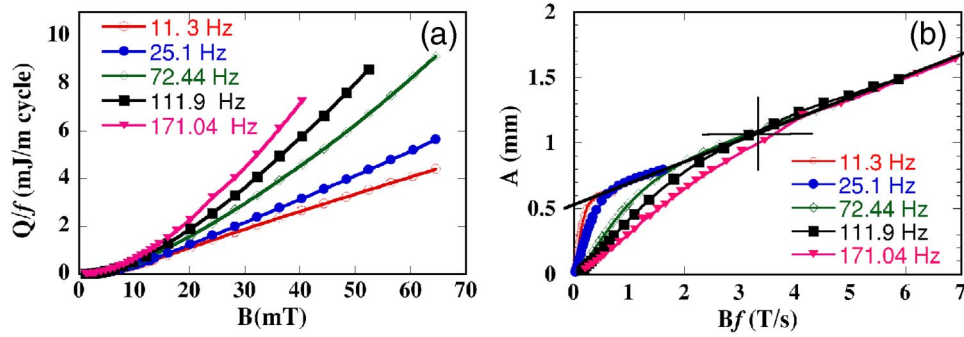
FIG. 2. (Color online) (a) The energy loss per cycle ( Q/f ) in the 20-filament sample, plotted vs amplitude of the applied magnetic field. (b) The specific loss \Lambda \equiv Q/I_c Bf in mm vs sweep rate. The plot includes all the data from (a). The loss data were normalized by a constant value of measured transport current I_c = 110 A. The straight line is an approximate linear fit corresponding to Eq. (5). Crossed lines in the center indicate the break-even point, where the coupling losses are equal to hysteresis loss.
