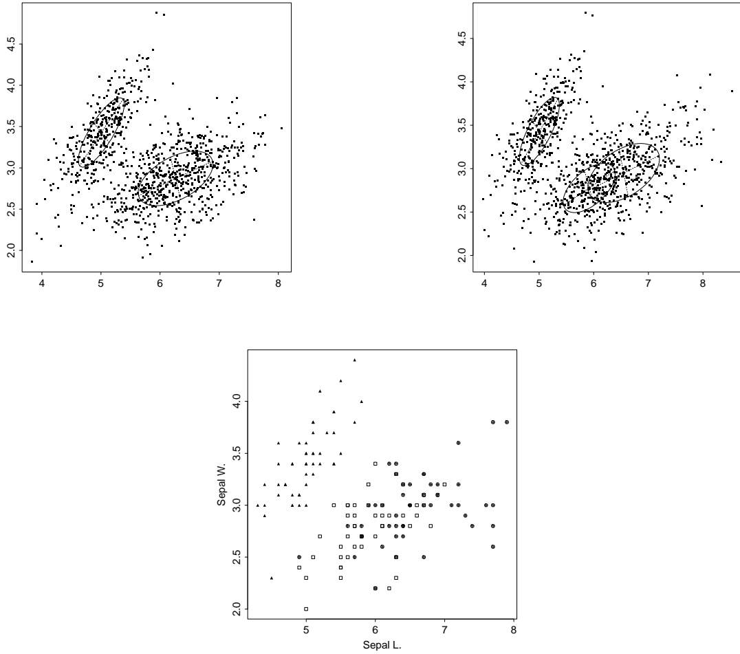
Figure 6: A projection of data simulated from EMclust models for Fisher's iris data. Upper Left: 1000 data points simulated from the 2-component VEV model. Upper Right: 1000 data points simulated from the 3-component VEV model. Lower: Fisher's iris data showing classification.
