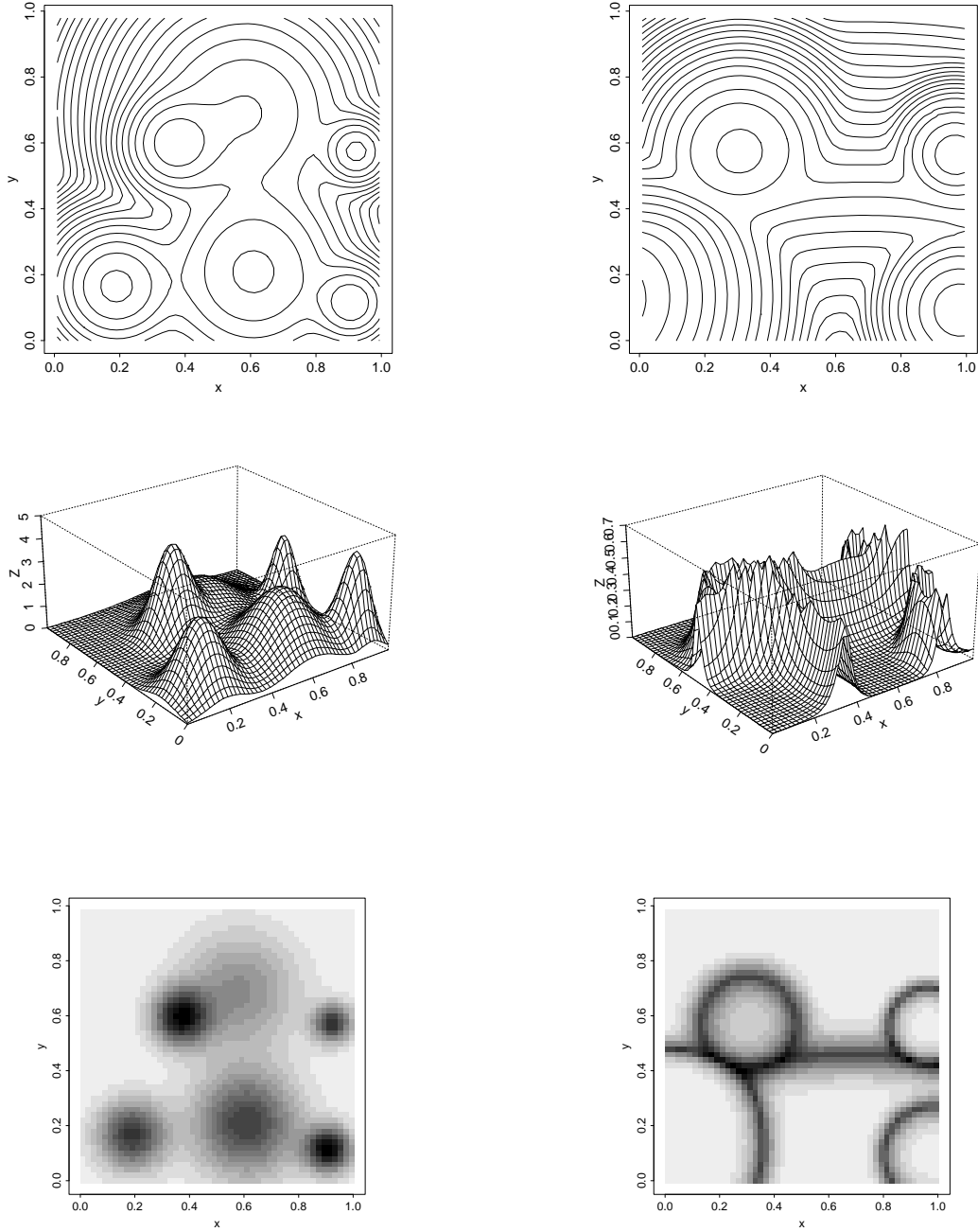
Figure 11: Density (left column) and uncertainty (right column) surfaces for the Lansing Woods maples. Contour, perspective, and image plots are displayed in the first, second, and third rows respectively. A logarithmic scale was used for the contour plots.
