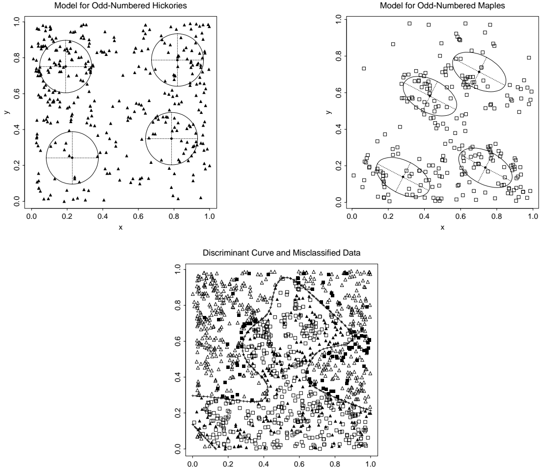
Figure 17: mclustDA models and discriminant curve for the Lansing Woods data. Upper Left: Model for the training [odd-numbered] hickories. Upper Right: Model for the training [odd-numbered] maples. Lower: discriminant curve with training and test errors (filled symbols). Note the small piece of the curve in the lower left-hand corner.
