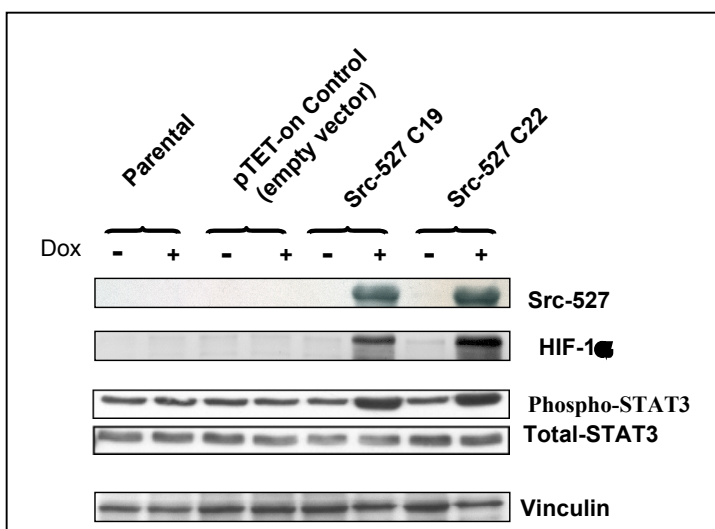
Figure 5. Induction of Src in "Tet-on" Clones leads to Increased HIF-1 \alpha Levels and PhosphoSTAT3. Inducible and control clones were described in last year's progress report. Here we show that STAT 3 and Hif phosphorylation increase, which as described below, is critical to increased VEGF expression.
