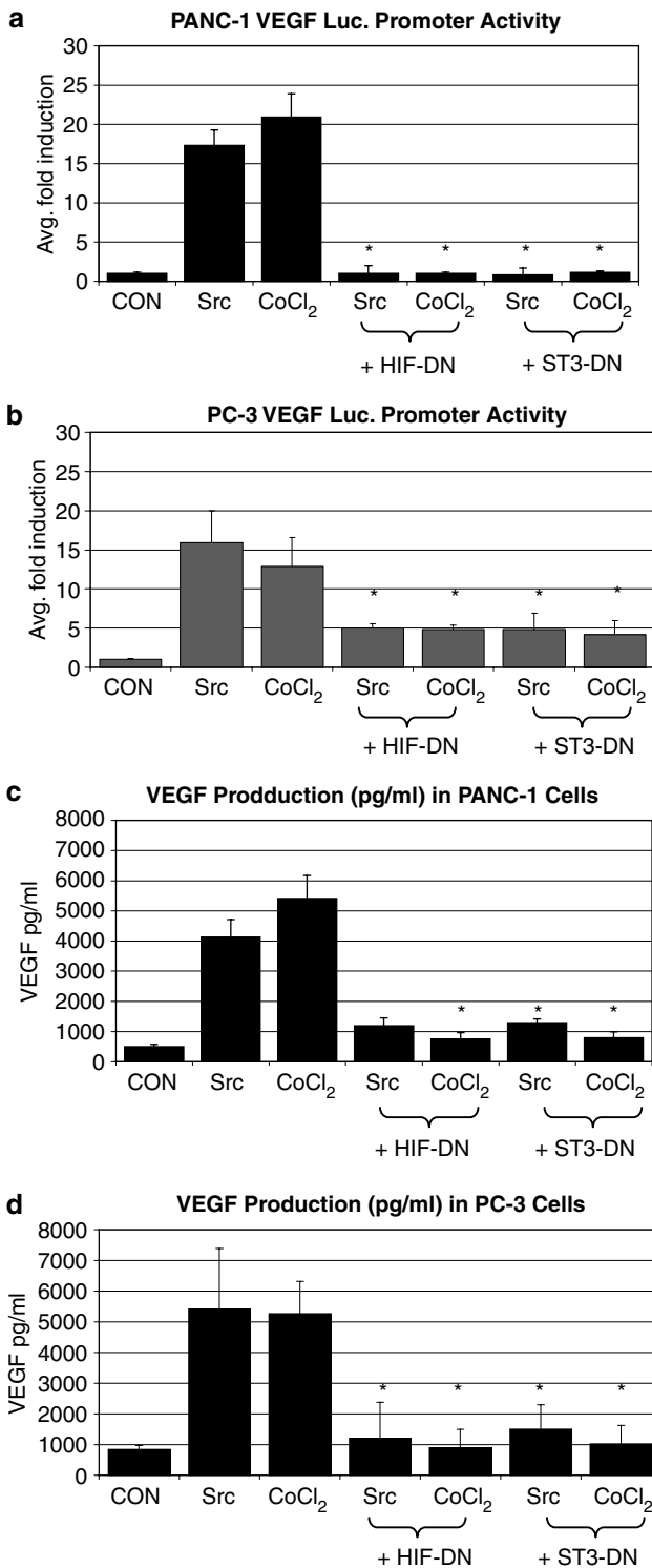
Figure 5 Dependence of activated HIF1 \alpha and phospho-STAT3 on transcription and expression of VEGF. Luciferase activity was determined in (a) PANC-1 cells and (b) PC-3 cells with or without expression of the indicated dominant negative mutant utilizing a luciferase reporter plasmid containing 2.2 kb of the human VEGF promoter. Cells were seeded in 12-well plates (0.25 \times 10 6 cells/well) and grown in complete media. Following a 24 h recovery period, cells were transfected with 200 ng of VEGF reporter plasmid and either 1.3 \mu g of pCEP4 (control wells), 1.3 \mu g of HIF-1 \alpha -DN plasmid (HIF-1 \alpha dominant negative), or 1.3 \mu g of STAT3-DN (STAT3 dominant negative) plasmid as indicated. Cells were treated 16 h later with CoCl 2 (100 \mu M) or doxycycline for 24 h at which time the medium was removed and stored at -80°C for ELISA and cells were lysed. Aliquots (20- \mu l) of each sample were analysed for luciferase expression and expressed as RLU. Relative luminescence was calculated as average luciferase activity (RLU)/protein concentration. All transfections were performed in triplicate. Asterisks denote significant differences ( P < 0.05 ) from columns with activated Src and treatment with CoCl 2 (c) VEGF expression in culture supernatants of PANC-1 cells and (d) PC-3 cells. From the above-described conditions, the medium was removed from cells and stored at -80°C. VEGF in the culture supernatants was determined by ELISA as described in Materials and methods. Asterisks denote significant differences ( P < 0.05 ) from columns with activated Src and treatment with CoCl 2
