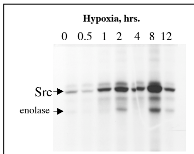
Figure 3. Induction of Src kinase Activity by Hypoxia. PC3-LN4 cells were placed in a hypoxia chamber (1% oxygen) for indicated times. Src kinase activity was measured by the immune complex kinase assay with enolase added as an exogenous substrate.
