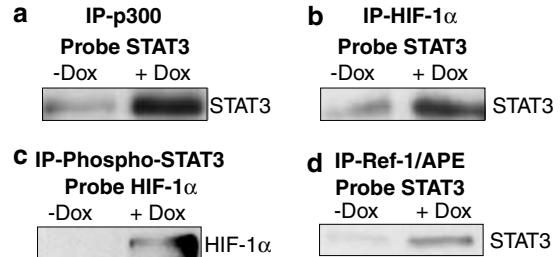
Figure 6 Coimmunoprecipitation of transcription factors after Src induction. Nuclear extracts were prepared from untreated and doxycycline treated (2 \mu g/ml, 24 h) PANC-1 tet-on Src-527 and immunoprecipitations were performed as described in Materials and methods. (a) Immunoprecipitation with an anti-p300 antibody and blot probed for STAT3. (b) Immunoprecipitation with an anti-HIF-1 \alpha antibody and blot probed for STAT3. (c) Immunoprecipitation with an anti-phospho-STAT3 antibody and blot probed for HIF-1 \alpha . (d) Immunoprecipitation with an anti-Ref-1/APE antibody and blot probed for STAT3
