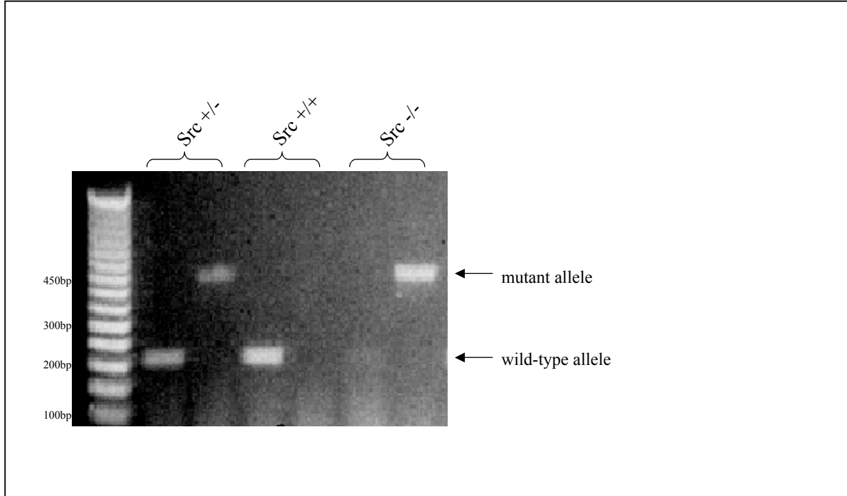
Fig. 9. Analysis of Src Alleles from DNA of Tail Snips of offspring of Src +/- parents after 6 back breedings into an nu/nu background. (A) indicates that wild type and mutant alleles can be identified from offspring. (B) 1 \times 10^6 PC3 cells were injected into the flank of one of the nu/nu offspring that formed a large tumor in six weeks. These results demonstrate the ability to grow human tumors in the Src-/- nude mice.
