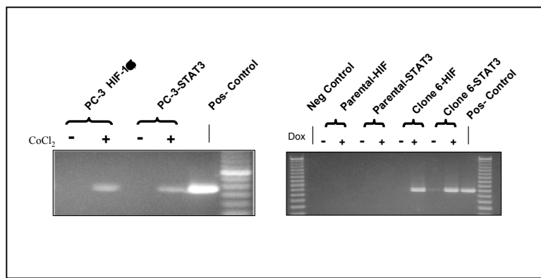
Figure 6. STAT3 and HIF bind at the same 350bp VEGF Promoter Fragment. Chromatin immunoprecipitation assays were performed on extracts from CoCl 2 or doxycycline- treated cells as described in the text. Both conditions led to increased amplification of the VEGF promoter fragment.
