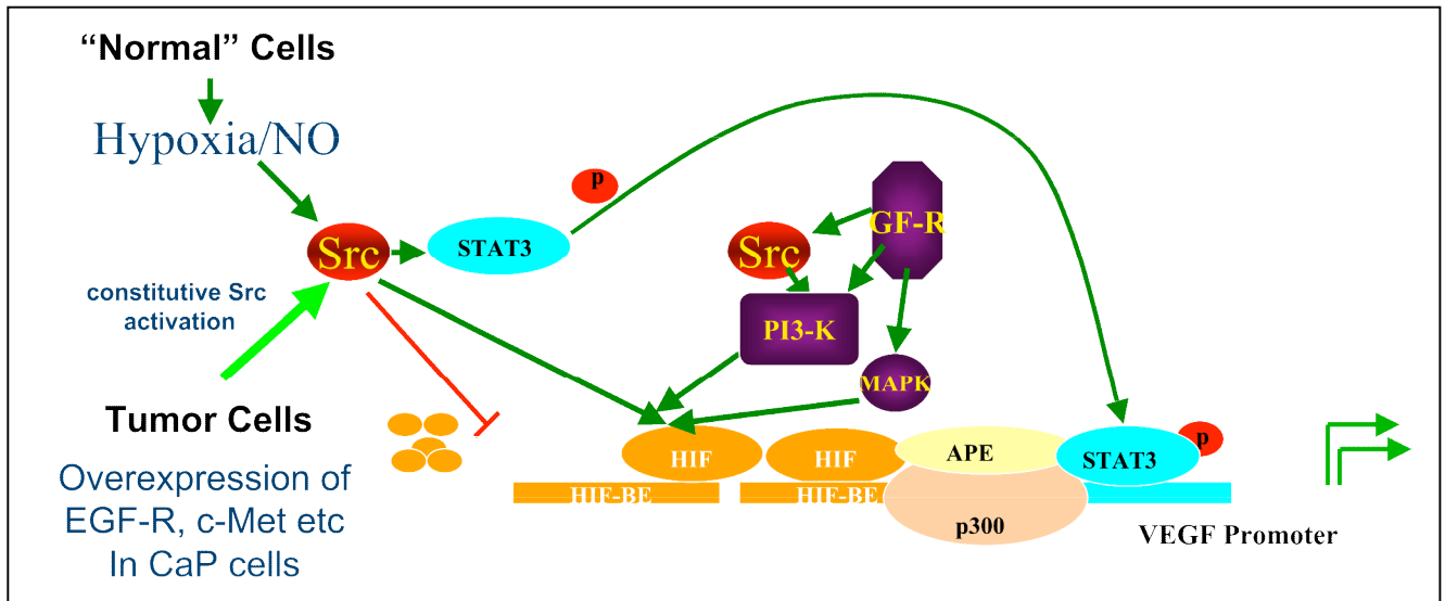
Fig. 8. Model from TASK 1: Src regulates VEGF Expression in Prostate Tumor Cells. In normal cells, hypoxia or Nitric Oxide (NO) leads to Src activation, which then leads to STAT3 phosphorylation, increasing VEGF transcription and subsequent production of this angiogenic factor. However, when Src is activated in later stage prostate tumors (lower left), this pathway is deregulated, increasing VEGF expression without the requirement for hypoxia or other stresses. This is the first demonstration of how Src activation can lead to prostate tumor progression, a main goal of studies in this proposal.
