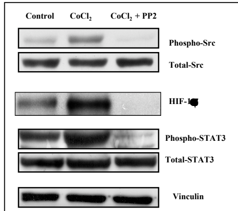
Figure 4. Cobalt Chloride Induces STAT3 phosphorylation and increases HIF-1 \alpha Steady-state Levels. PC-3 cells were treated with CoCl 2 with or without PP2 as described in the text. Increased phosphorylation of Src on Y418 (i.e. activation) is required for STAT3 phosphorylation and increased HIF-1 \alpha expression.
