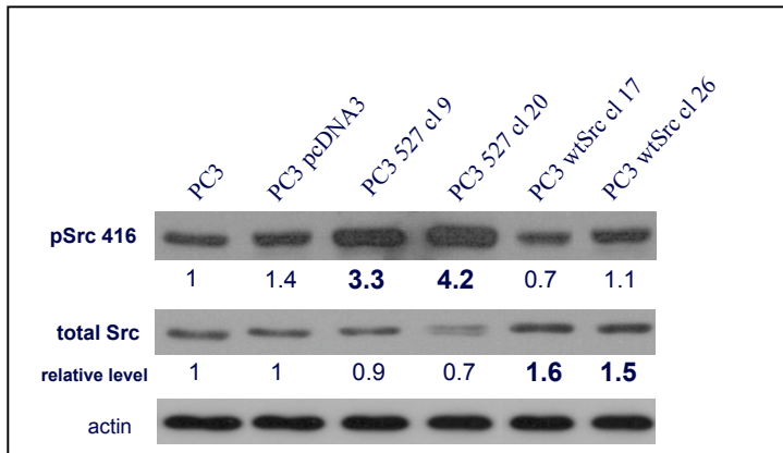
Fig. 1. PC3 cells were transfected with vector alone, or vector expressing Y527F activated Src or wild type Src. Individual clones were expanded and immunoblotting for activated Src with an antibody to \gamma -P416 or total Src was performed. Actin is used as a loading control. Numbers represent increased Src expression over vector control.
