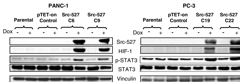
Figure 2 Effect of induction of activated Src on HIF1α expression and STAT3 phosphorylation. Parental, empty vector controls, or tet-on Src-527-expressing cells lines were grown and incubated with and without doxycycline (2 ng/ml) 24 h prior to cell lysis as described in Materials and methods. Expression of activated Src was ascertained by immunoblotting with an avian-specific Src antibody (EC-10). In addition, immunoblotting with HIF-1α, phospho-STAT3, and total STAT3 was performed. Immunoblots were reprobbed with an antibody to vinculin as a loading control
