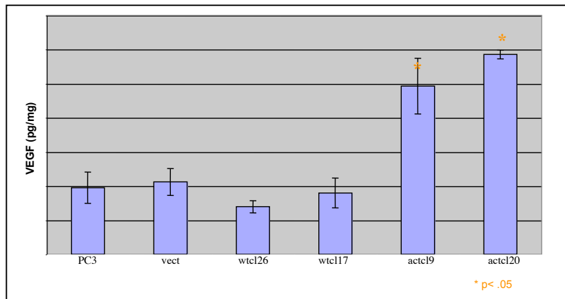
Fig. 2. VEGF expression in supernatants from parental PC3, vector control, and clones overexpressing wild type or activated Src. VEGF was measured by ELISA assay.
