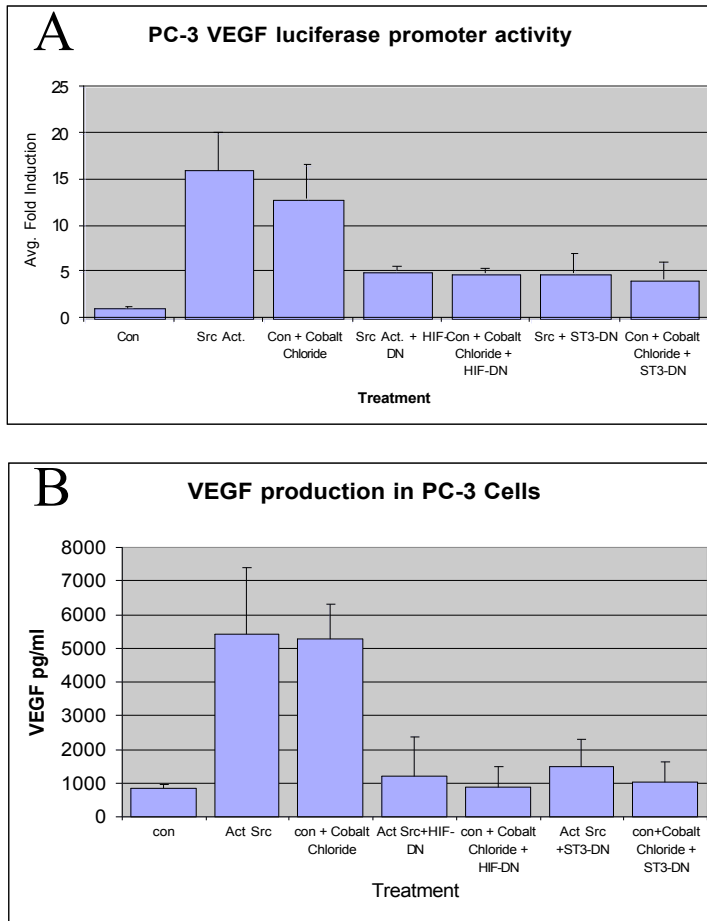
Fig. 7. VEGF expression is inhibited by either a dominant negative STAT3 or HIF-1a. A. VEGF promoter activity was estimated by a luciferase assay as described in the text. Displayed are results from both dominant negative mutants following Src induction in Tet-on clone 6 "Src-Act" of following cobalt chloride treatment. B. VEGF levels in supernatants used in A were determined by ELISA .
