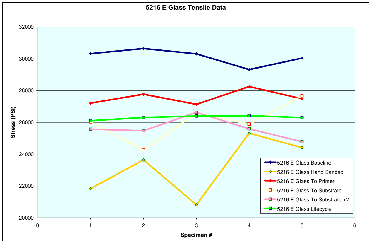
Figure 22. Tensile test results for 5216 E glass.
