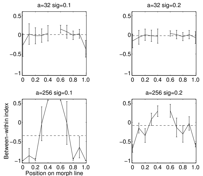
Figure 5: Mean between-within index (BWI) of view-tuned units with preferred stimuli spaced along the morph lines. Error bars show standard deviation across the nine morph lines.
