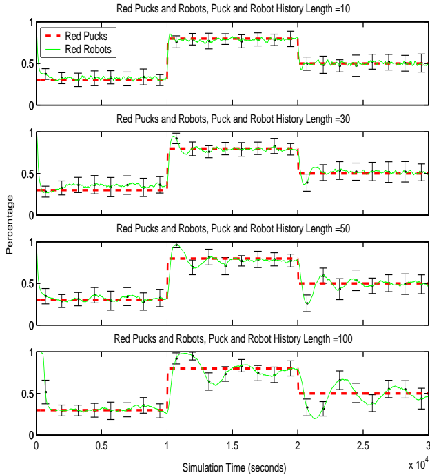
Fig. 1. Proportion of Puck Red pucks and robots foraging for Puck Red pucks over time when using the probabilistic transition function and different puck and robot history lengths, shown with 1 standard deviation error bars.
