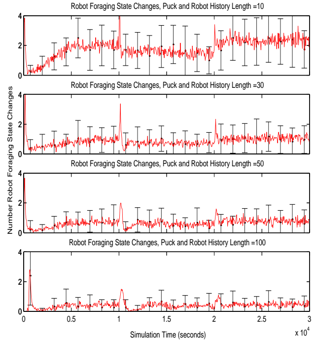
Fig. 2. The number of foraging state changes when using the probabilistic transition function and different puck and robot history lengths, shown with 1 standard deviation error bars.
