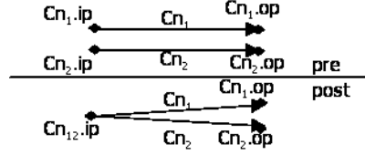
Fig. 11. Port Aggregation PortAgg2 Pattern
