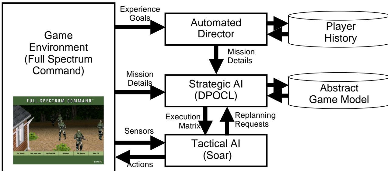
Figure 1: The Adaptive Opponent Architecture.
