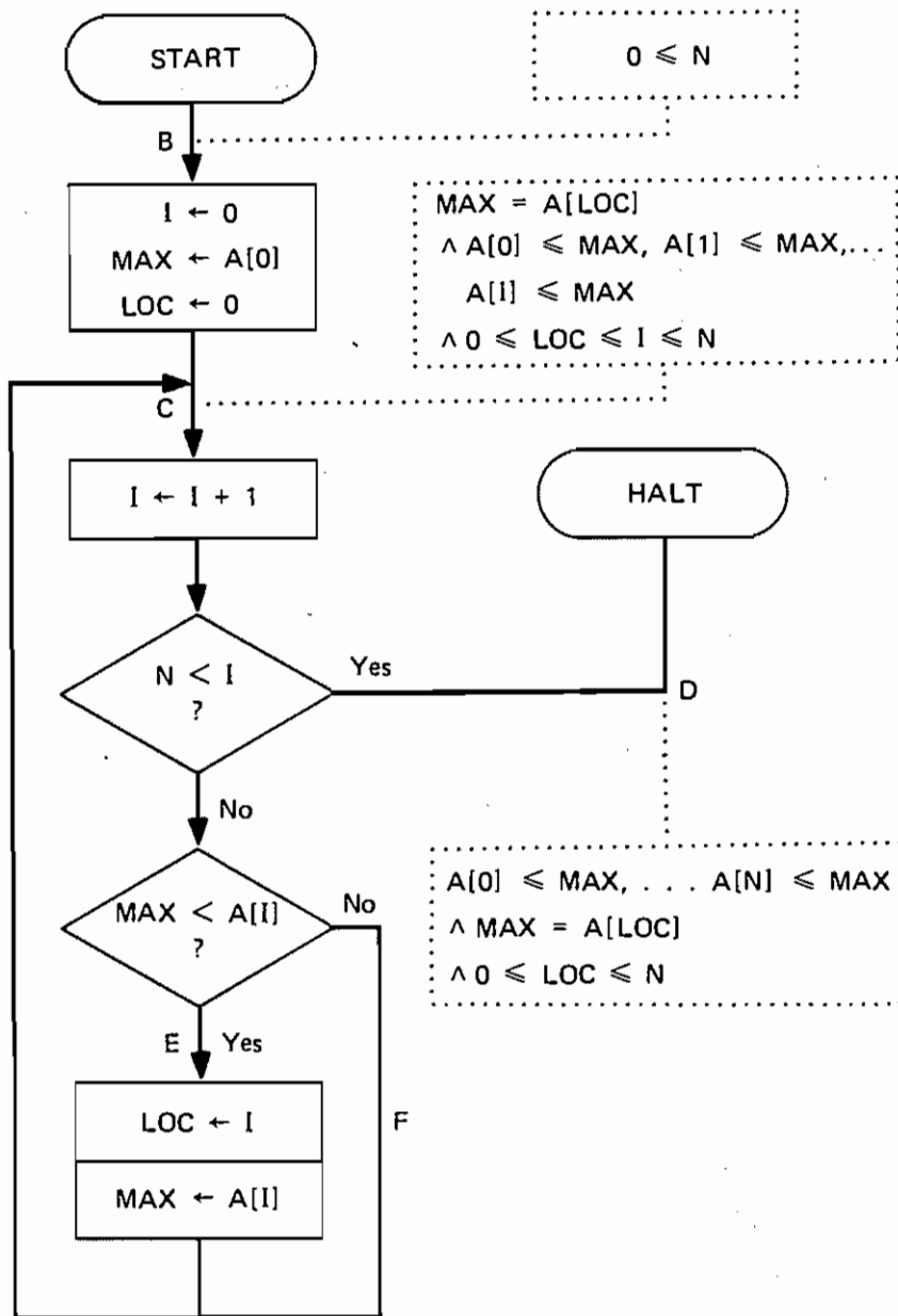
FIGURE 1 FINDING THE MAXIMUM OF AN ARRAY.
