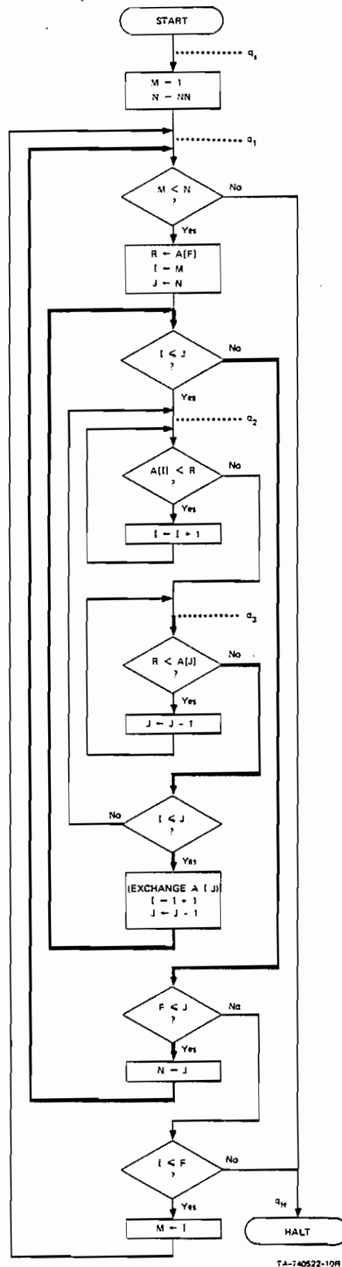
FIGURE 3 THE FIND PROGRAM
